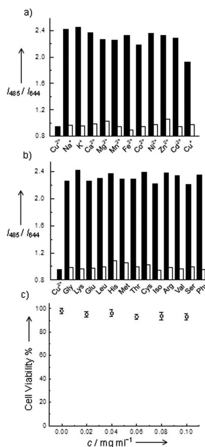
Figure 3. a) Fluorescence responses of CdSe@C-TPEA towards various metal ions. The black bars represent the addition of an excess of metal ions (1 mM for Na + , K + , Ca 2+ , and Mg 2+ ; 50 \mu M for other cations) to a 0.02 mg mL -1 solution of CdSe@C-TPEA (pH 7.4). The white bars represent the subsequent addition of 50 \mu M Cu 2+ ions to the solution. b) Fluorescence responses of CdSe@C-TPEA toward various amino acids. The black bars represent the addition of 100 \mu M amino acid to a 0.02 mg mL -1 solution of CdSe@C-TPEA (pH 7.4). The white bars represent the subsequent addition of 50 \mu M Cu 2+ ions to the solution. The excitation wavelength was set to 400 nm. c) Cell viability values (%) estimated by MTT proliferation tests versus incubation concentrations of CdSe@C-TPEA (0, 0.02, 0.04, 0.06, 0.08, 0.1 mg mL -1 ) at 310 K for 24 h.
