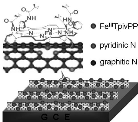
Figure 1. Proposed schematic diagram of the \text{CN}_x MWNTs/FeTpivPP-modified GCE.
