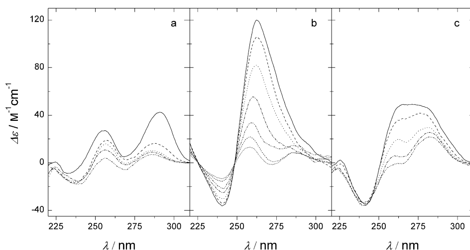
Figure 7. Thermal denaturation of the structures formed in the presence of [\text{Ru}(\text{NH}_3)_6]^{2+} . CD spectra of: a) TBA, b) GTAGGT-TBA, and c) TTTTTT-TBA in Tris buffer (pH 7.4) in the presence of 10 equiv [\text{Ru}(\text{NH}_3)_6]^{2+} measured every 10 °C starting from 5 °C (solid line).
