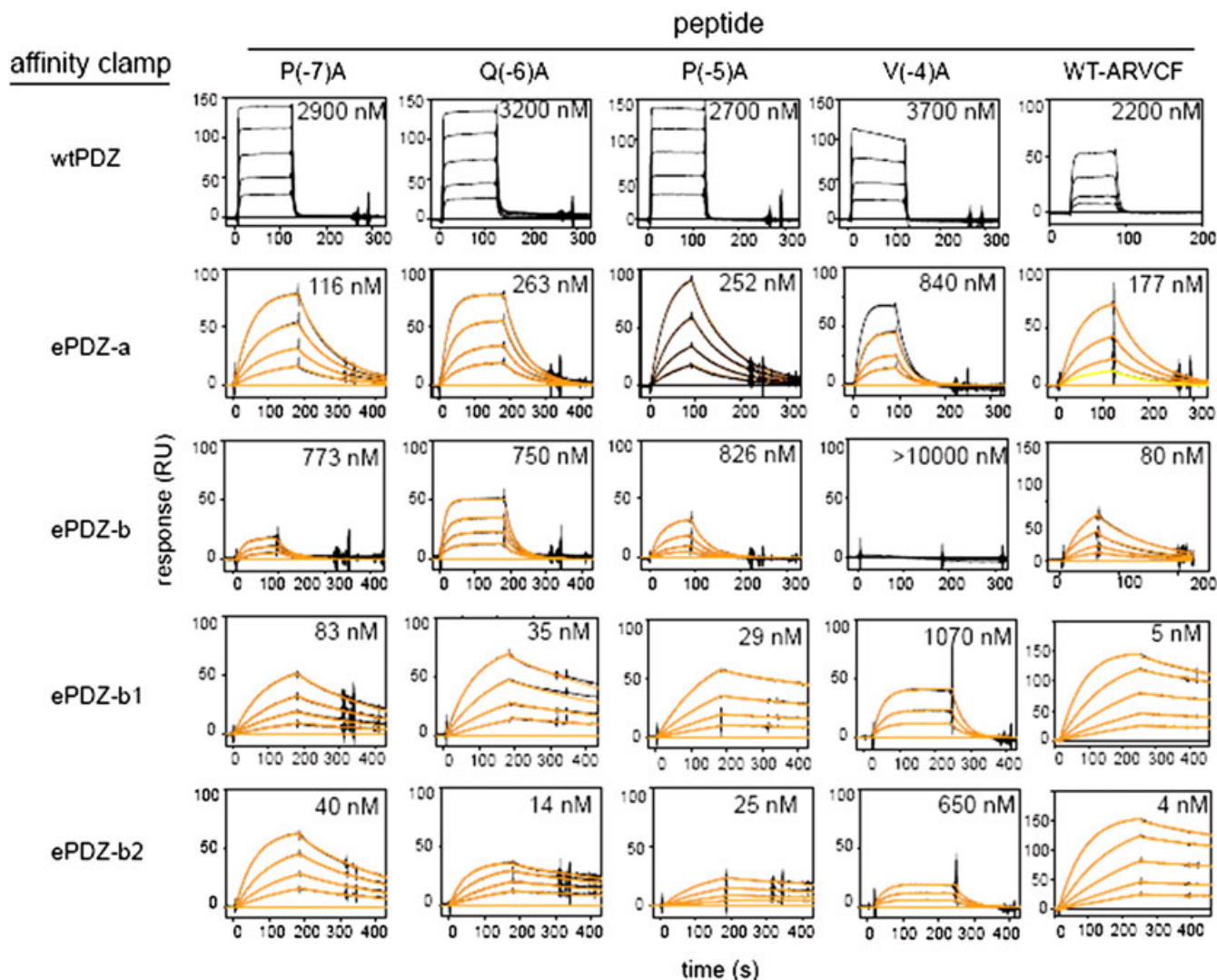
Figure 6. Responses and fits for Ala-substituted peptides binding to successive generations (from top to bottom) of engineered proteins. The fit of the 1:1 interaction model is overlaid atop each data set fit using kinetic analysis. Affinities of the weakest interactions (top row) were determined using equilibrium analysis. Reprinted from reference 68 with permission from Elsevier © 2009.
