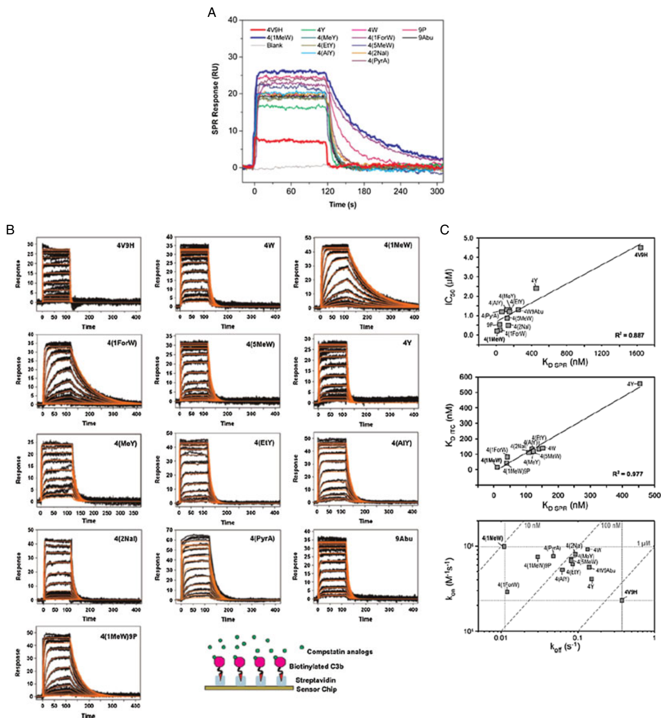
Figure 7. Structural modifications in compstatin that affect its binding to C3b. (A) Kinetic screening of compstatin analogs. Thirteen peptides were tested at the same concentration for binding to surface-tethered C3b. (B) Full kinetic analyses of the 13 analog/C3b interactions. Red lines depict the fit of the responses (duplicates at each compstatin concentration) to a 1:1 interaction model. A cartoon illustrating the assay design is included at the bottom of the panel. (C) Correlations between binding parameters. Top: activity (half maximal inhibitory concentration [ IC_{50} ], ELISA) versus affinity ( K_D , SPR); middle: solution-determined affinity ( K_D , ITC) versus surface-determined affinity ( K_D , SPR); bottom: k_a versus k_d , with dashed isoaffinity lines included. K_D =equilibrium dissociation constant; k_a =association rate constant; k_d =dissociation rate constant. Reprinted from reference 96 with permission from John Wiley & Sons, Ltd. © 2009.
