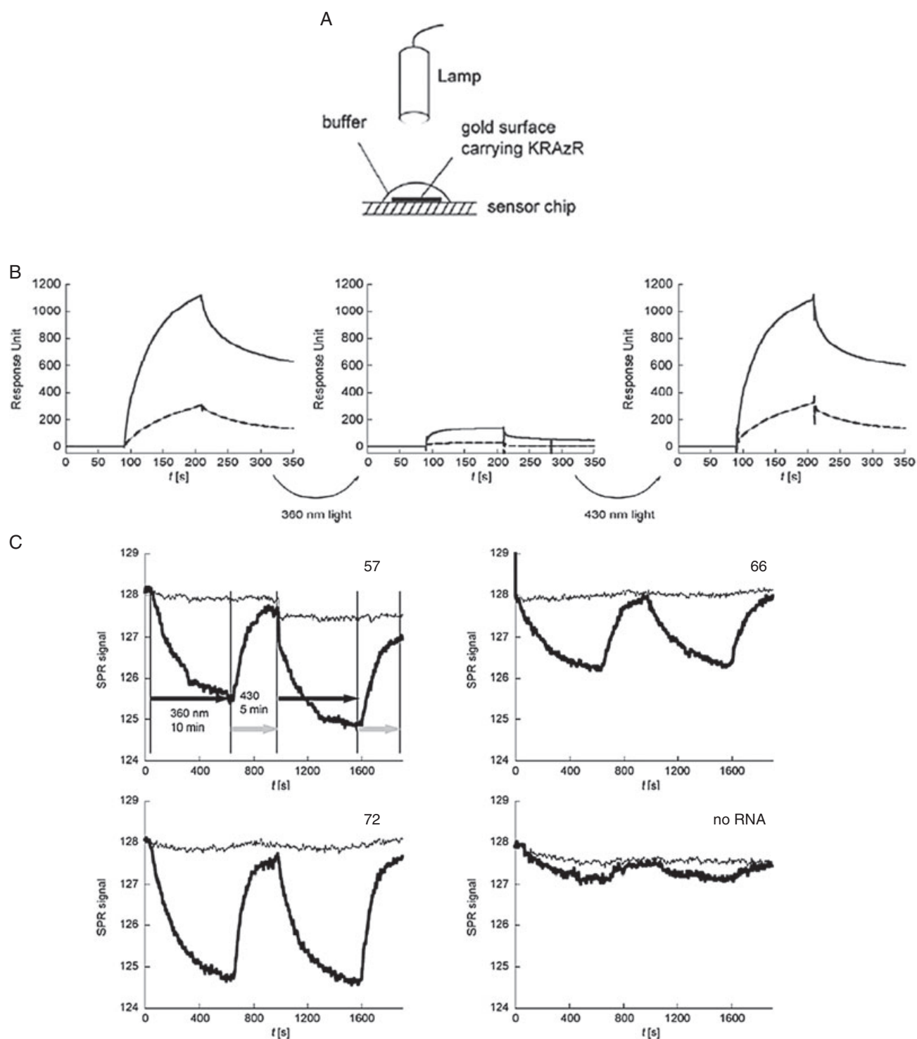
Figure 10. RNA binding to a photoresponsive peptide, KRAzR. (A) Off-line irradiation of peptide immobilized on a Biacore sensor chip. (B) Responses obtained using Biacore 2000 for two aptamers (indicated by the solid and dashed lines) injected across the peptide surface before (left) and after photoirradiation at 360 nm (middle) and 430 nm (right). (C) Real-time monitoring using Toyobo SPR-200 of the photoresponsiveness of three aptamers (designated 57, 66, and 72) binding to KRAzR. The bottom right panel shows the signals obtained for a buffer blank test. In each panel, the thin gray lines depict the signals from reference positions on the sensor surface. Reprinted from reference 229 with permission from Wiley-VCH Verlag GmbH & Co. © 2009.
