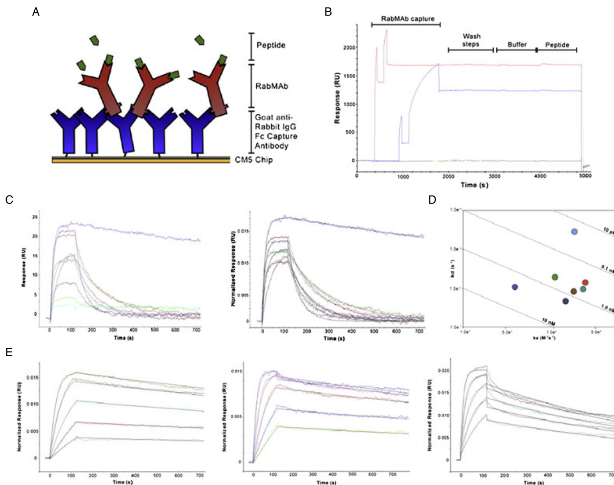
Figure 9. Ranking anti-peptide antibodies from hybridoma supernatants. (A) Assay design for the kinetic screening of anti-peptide RabMAbs. (B) Full binding cycle for the testing of two RabMAbs. (C) Overlay of representative peptide binding responses (left) and the fit of these responses (normalized for capture level) to a 1:1 interaction model (right). Responses of <5 resonance units in the left panel were omitted from the kinetic fitting. (D) Kinetic distribution plot of selected RabMAbs. Diagonal lines depict affinity isotherms. (E) Rigorous kinetic analyses of three RabMAb/peptide interactions. Reprinted from reference 115 with permission from Elsevier © 2009.
