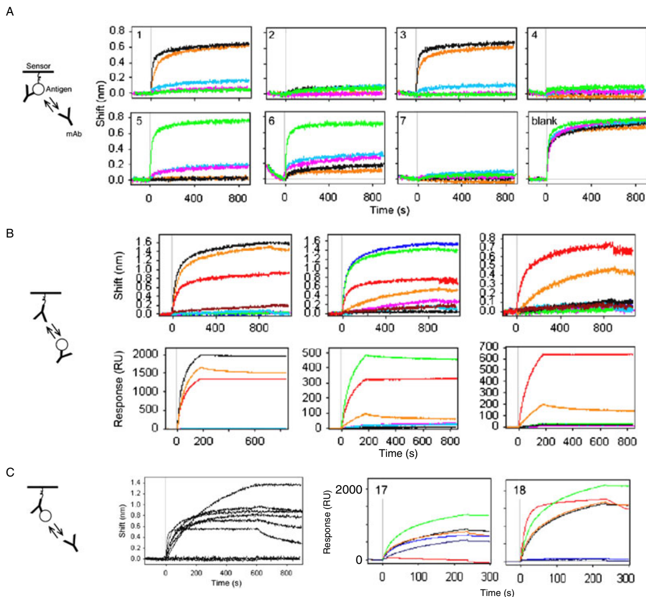
Figure 3. Epitope binning with three assay formats. (A) In tandem blocking of competing mAbs in solution screened against pre-formed Ag/mAb complexes measured using Octet QK. (B) Premix blocking of Ag/mAb complexes in solution screened against three immobilized mAbs (left to right) measured using Octet QK (top) and ProteOnXP36 (bottom). (C) Responses from a classical sandwich format for mAbs screened using the Octet OK (left) and ProteOnXPR36 (right). Reprinted from reference 200 with permission from Elsevier © 2009.
