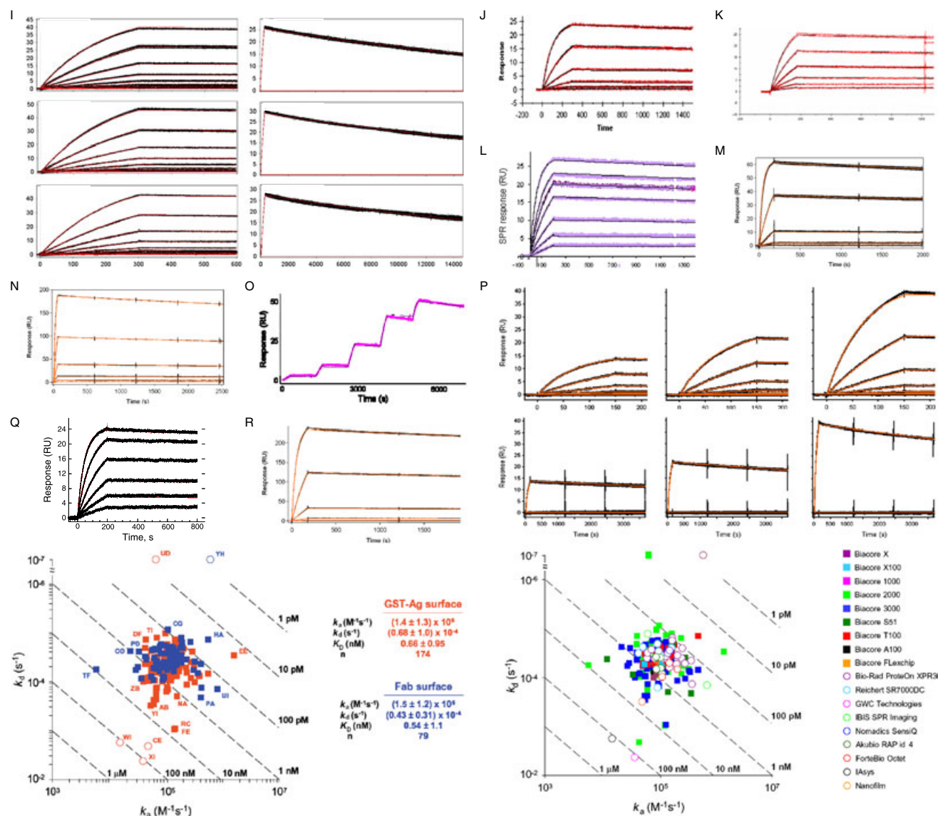
Figure 11. Global benchmark study. (top) Data sets collected by participants I through R. (bottom) k_d versus k_a plots of the kinetic parameters determined by the participants. (bottom left) Analyses of Ag surfaces are shown in red, and Fab surface are shown in blue. (bottom right) Analyses grouped by biosensor platform. Reprinted from reference 122 with permission from Elsevier © 2009.
