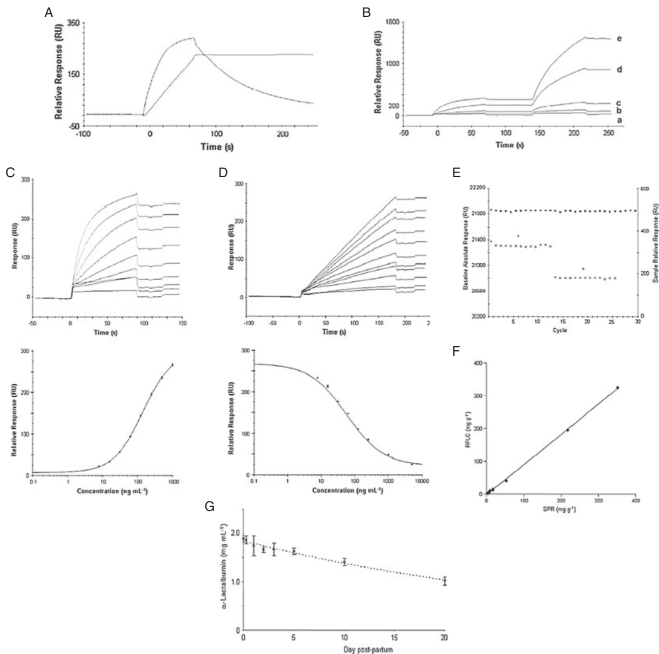
Figure 2. Development of an \alpha -lactalbumin immunoassay. (A) Screen of two \alpha -lactalbumin binders. (B) Enhanced binding approach: injections of five \alpha -lactalbumin concentrations (a–e) followed by injections of anti- \alpha -lactalbumin across an \alpha -lactalbumin surface. (C) Responses and isotherm obtained from the direct binding assay. (D) Responses and dose-dependent curve from the inhibition assay. (E) Reproducibility of replicate tests of (a) \alpha -lactalbumin standard and (b) whey protein isolate. The responses from the baseline are included as a reference (filled squares). (F) Correlation between the \alpha -lactalbumin detected by biosensor and reverse-phase liquid chromatography. (G) Biosensor-determined bovine \alpha -lactalbumin content in early lactation milk. Reprinted from reference 189 with permission from Elsevier © 2009.
