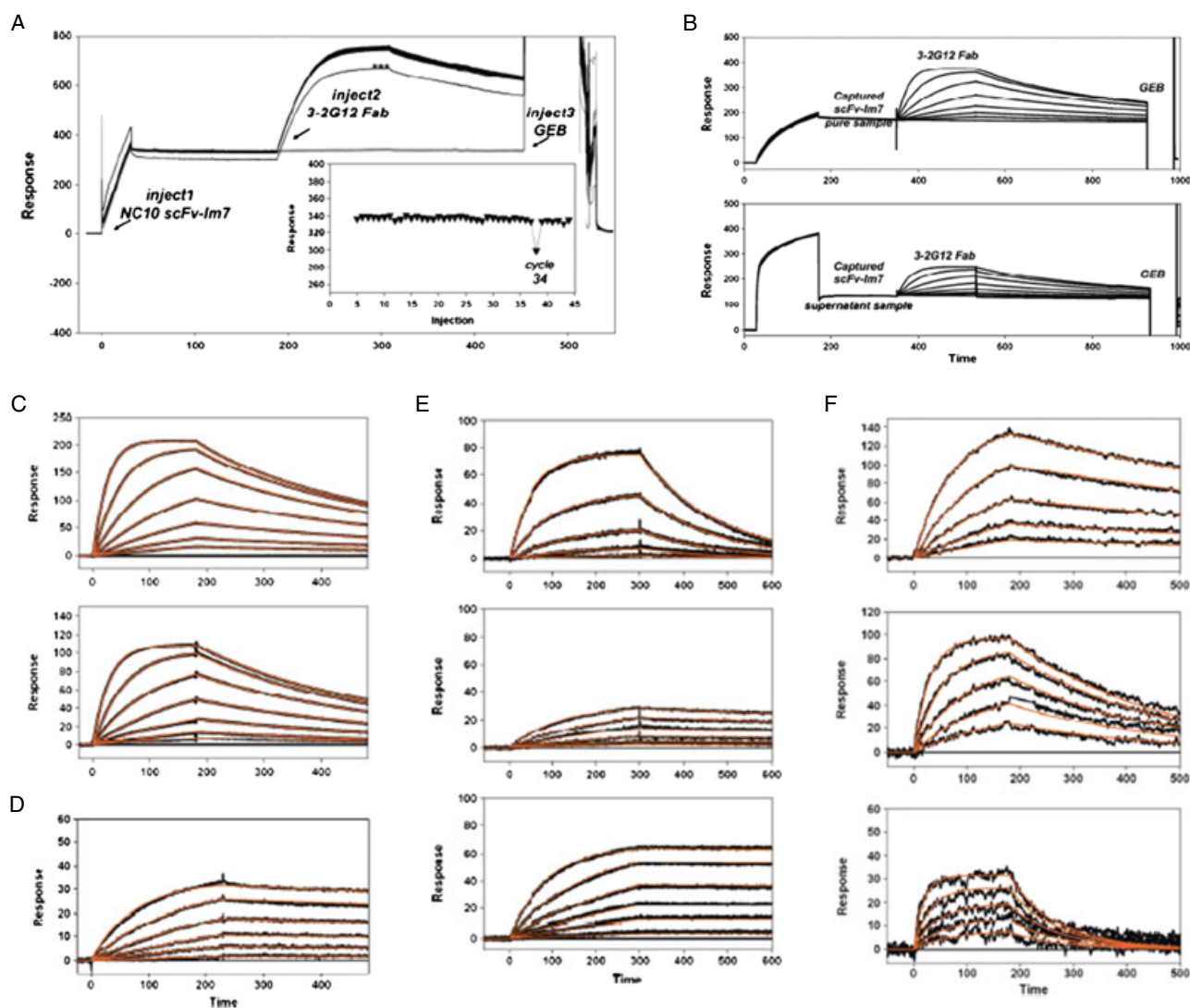
Figure 4. Capture and kinetic analyses of Im7 conjugates. (A) Reproducibility of NC10 scFv-Im7 capture and activity. (B) Overlay of full binding cycles of a 3-2G12 Fab concentration series binding to purified and crude preparations of NC10 scFv-Im7. (C) Responses for 3-2G12 binding to captured NC10 scFv-Im7 (affinity-purified, top panel; crude, bottom) fit to a 1:1 interaction model (red lines). (D) Carcinoembryonic antigen binding to captured T84.66 scFv2-Im7 diabody. (E) Ricin binding to three anti-ricin Fab-Im7s captured from culture supernatants. (F) Apical membrane antigen 1 binding to three captured 12Y-2 V_{\text{NAR}} -Im7 clones. Data in panels A-E were collected using Biacore T100; data in panel F were collected using BioRad ProteOn XPR36. Reprinted from reference 67 with permission from Elsevier © 2009.
