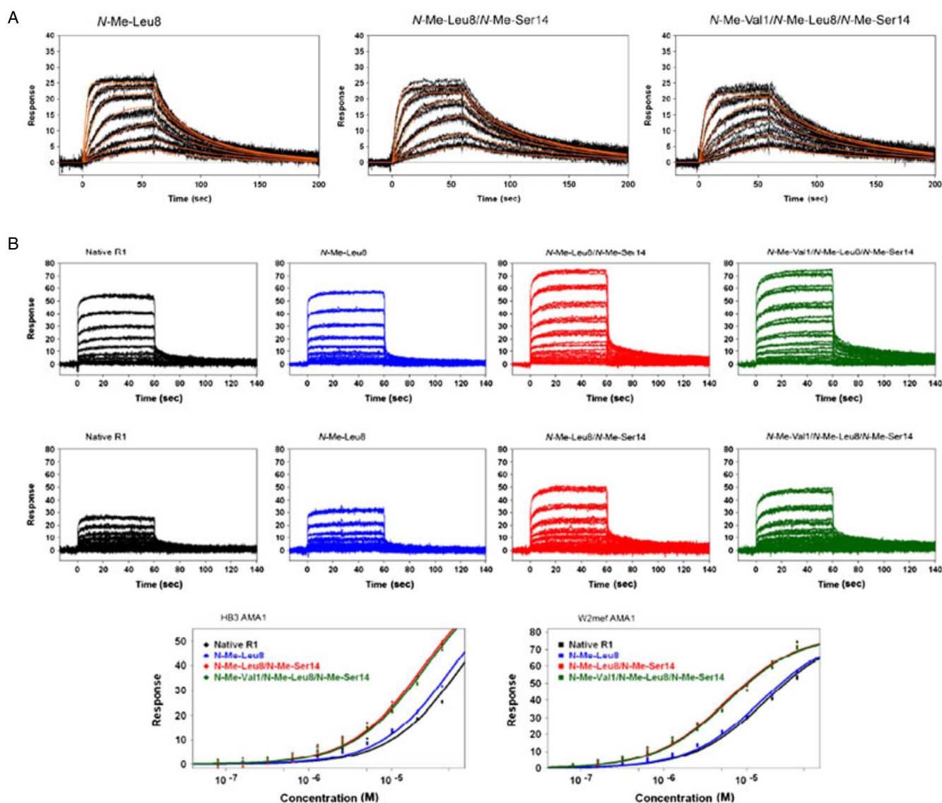
Figure 5. Kinetic and equilibrium analyses of native and mutated R1 peptides binding to immobilized AMA1. (A) The fit of a 1:1 interaction model is overlaid atop the responses collected for three mutant peptides/AMA1 interactions, with triplicate responses of each peptide concentration shown. (B) Triplicate responses (top) and isotherms (bottom) obtained for four weaker-affinity peptides binding to two forms of AMA1. Reprinted from reference 66 with permission from the American Society for Biochemistry and Molecular Biology © 2009.
