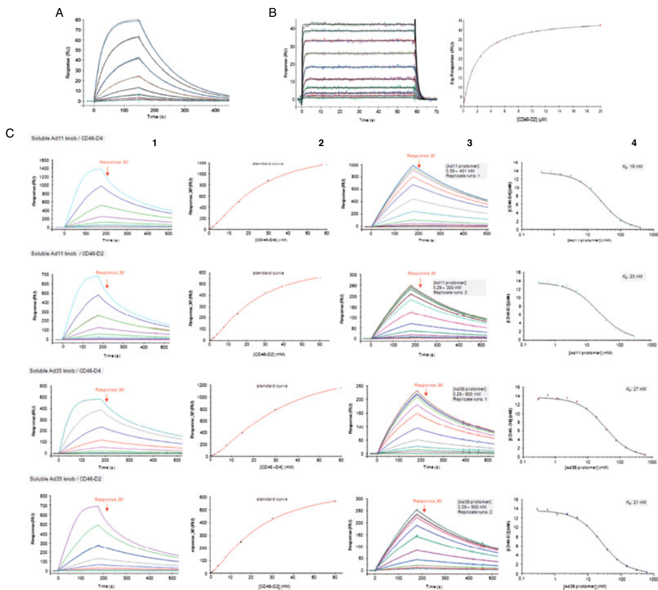
Figure 8. Analyses of CD46/Ad knob interactions. (A) Kinetic analysis of CD46 binding to immobilized Ad11 knob, with the fit of a 1:1 interaction model overlaid atop the duplicate responses obtained for each CD46 concentration. (B) Kinetic and equilibrium analyses of CD46 (tested in duplicate) binding to a mutant Ad11 knob surface. (C) The four steps (labeled 1–4 left to right) in solution-competition analyses of soluble Ad11 and Ad35 knobs competing with immobilized Ad35 for binding to CD46. Reprinted from reference 112 with permission from the American Society for Microbiology © 2009.
