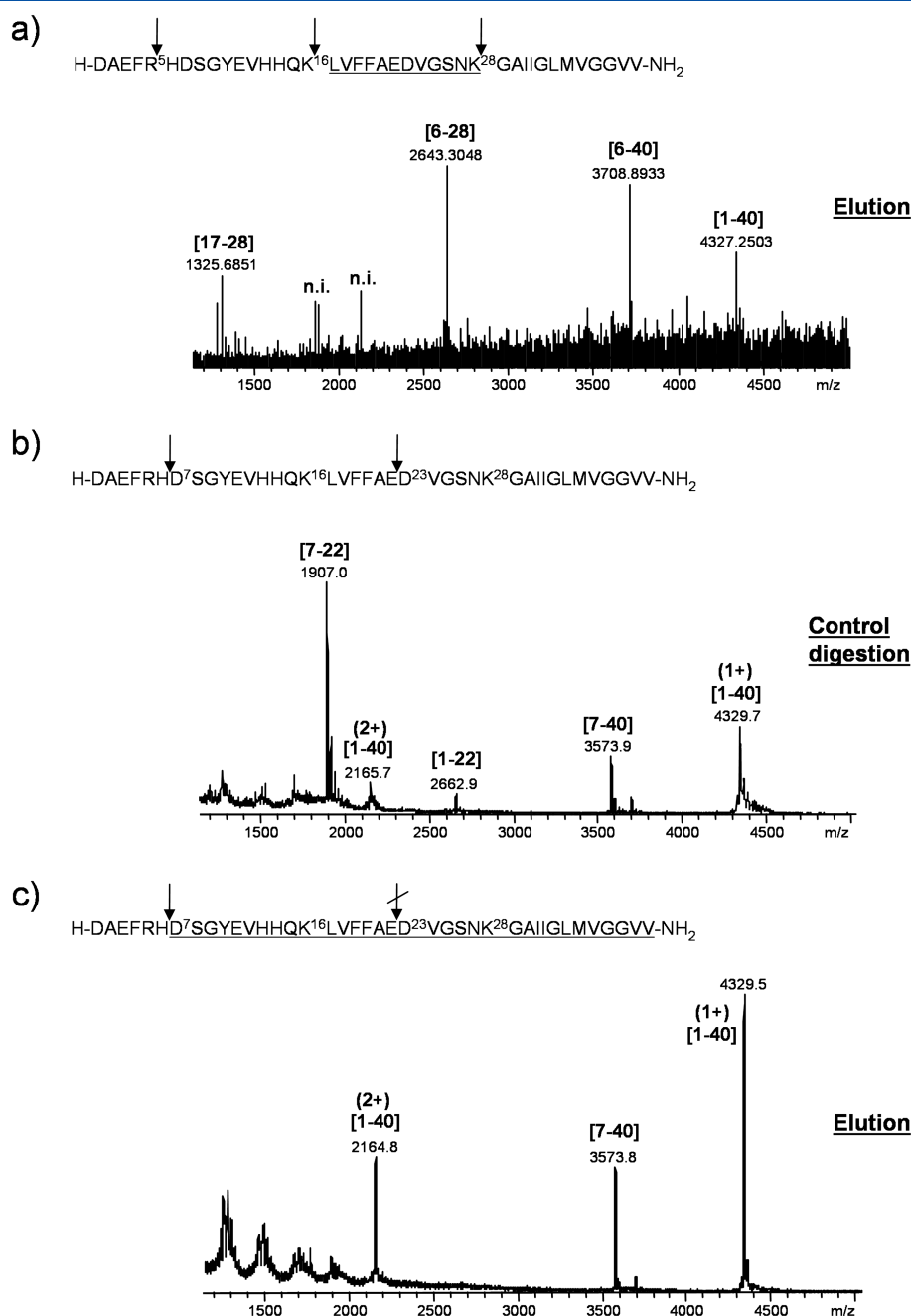
Figure 5. (A) MALDI-FTICR mass spectrum of the elution fraction after addition of trypsin-digested Aβ(1–40) on the HN affinity column (proteolytic extraction). The trypsin cleavage sites are indicated by arrows and the minimal epitope sequence Aβ(17–28) is underlined; n.i. not identified; (B) MALDI-TOF mass spectrum of the fragment peptides obtained after Asp-N digestion of free Aβ(1–40) in solution (control digestion). The Asp-N cleavage sites are indicated by arrows; (C) MALDI-TOF mass spectrum of the elution fraction obtained after proteolytic excision of Aβ(1–40) with Asp-N. The Asp-23, shielded from Asp-N digestion in the Aβ–HN complex, is indicated by a broken arrow and the Aβ(7–40) epitope sequence is underlined.
