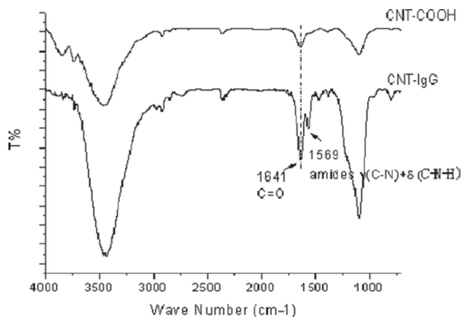
Fig. 3. ATR-FTIR spectra of CNTs. The absorption peak at 1,569 \text{cm}^{-1} indicates the presence of amide linkage between MWCNTs and IgG
