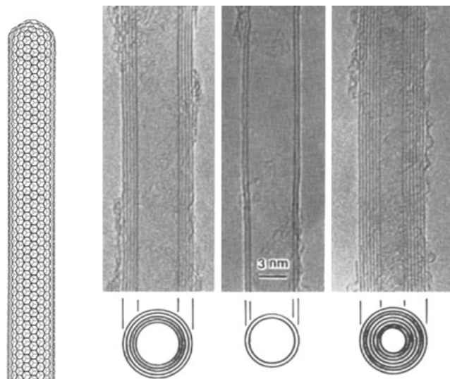
Fig. 3 A SWNT can be visualised as a rolled-up sheet of graphite capped by half of a C_{60} molecule (diagram on the left). CNTs can also exist as DWNTs and MWNTs. TEM images reveal the number of walls present (image on the right shows five, two and seven layers, respectively) [26]. Reproduced with permission from the Nature Publishing Group
