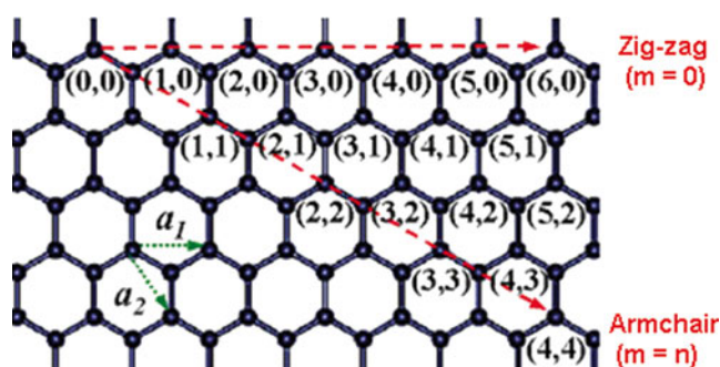
Fig. 4 Nanotubes possess an armchair, zigzag or chiral structure depending on the angle at which they are rolled up (this determines the n , m and \theta values)
