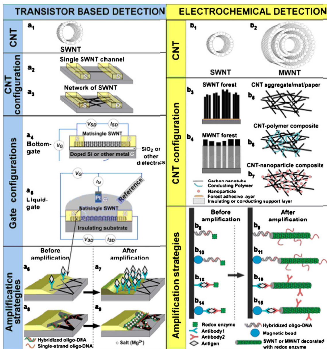
Fig. 8 Schematic representation of biomolecular sensing using carbon nanotubes in various device configuration and signal amplification strategies [114]. Reproduced with permission from Wiley-VCH Verlag GmbH
