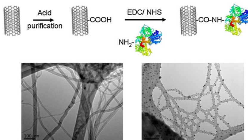
Fig. 5 Biomolecules can be covalently attached to acid functionalities on CNT surfaces via EDC/NHS coupling with amide groups on a biomolecule (scheme shown top). TEM can be used to effectively
