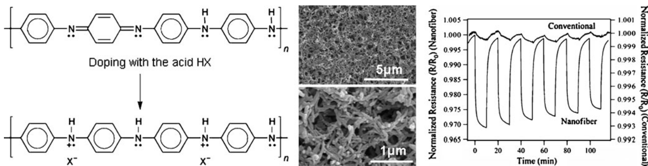
Fig. 7 The chemical bonding structure of CP-PANI is sensitive to the chemical environment of the material ( left ). In its nanoform, the material is more responsive than in the bulk form ( right shows sensing results, reproduced with permission from the American Chemical Society) [143]
