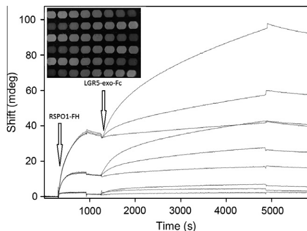
Fig. 1. A typical SPR overlay plot showing the loading of RSPO1-FH (300–900 s) on three spots with decreasing anti-Flag antibody densities ( R_{\text{RSPO1}} values of ~35, 12, and 2 mdeg) followed by three injections of LGR5-exo-Fc in serial dilution starting at 45 nM. The results of only three spots are shown for clear presentation, but the results of all eight spots were used to calculate the k_d^{\text{RO}} and K_D^{\text{RO}} values. Inset: Typical SPR image of 48 spots in a 6 \times 8 ligand density array printed by a Continuous Flow Microspotter.
