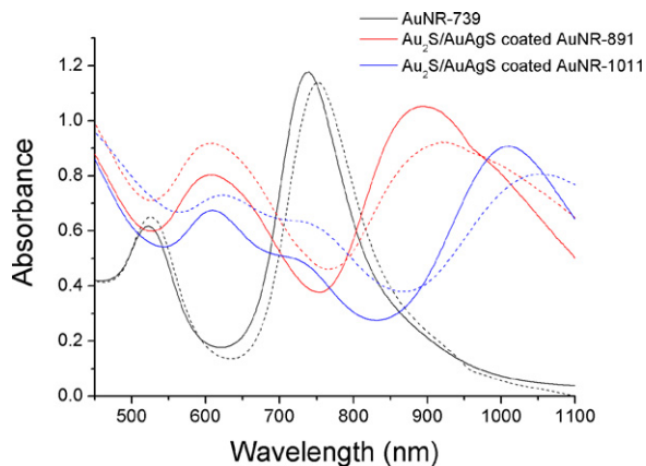
Fig. 4. Three pairs of absorption spectra corresponding to the three types of nanorods as shown in Fig. 2. Each pair shows that the red shift resulted from the recognition of rabbit anti-goat IgG with goat IgG attached on the different types of nanorods.
