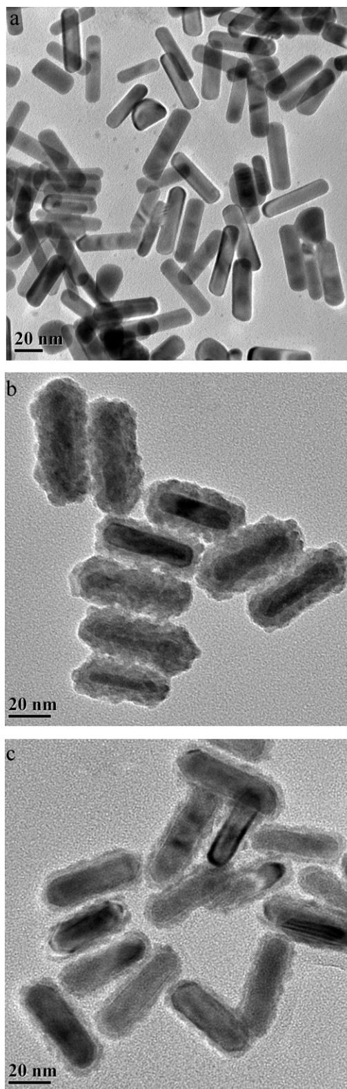
Fig. 2. TEM images of gold nanorods (a, LPW at 739 nm), the resulted composite gold nanorods (b, LPW at 891, and c, 1011 nm) at different stages.
