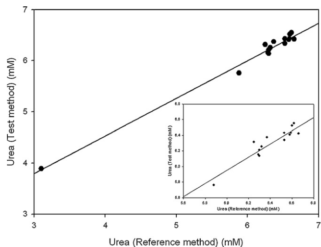
Fig. 4. Correlation of the nanoPANI/urease biosensor with a spectrophotometric enzyme assay kit for the determination of urea in 15 human serum samples. Intercept = 0.89, slope = 0.84 and r^2 = 0.85 . Inset shows the cluster of 14 samples from 5.8 to 6.8 mM.
