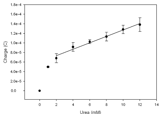
Fig. 3. Calibration of the nanoPANI/urease sensor after addition of urea, pre-incubation at 0.07 V for 150 s and stepped to -0.3 V vs. Ag/AgCl, followed by measurement of cathodic charge passed after 50 s ( n=3 ). From 2 to 12 mM, slope = 6.7 \mu\text{C mM}^{-1} , intercept = 60.1 \mu\text{C} , r^2 = 0.98 .
