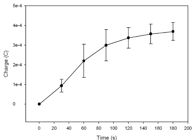
Fig. 2. The effect of time on the coulometric response from the nanoPANI/urease biosensor in the presence of 5 mM urea. Chronocoulometric response taken at 50 s following step potential from 0.07 V to -0.3 V vs. Ag/AgCl. All measurements were performed at 25 \pm 1 °C ( n=3 ).
