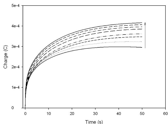
Fig. 1. Chronocoulometric response of the nanoPANI electrode to ammonium as ammonium chloride. Electrodes were poised at the equilibrium potential of 0.07 V vs. Ag/AgCl for 50 s upon the addition of the ammonium chloride and then stepped to -0.3 V vs. Ag/AgCl for 50 s over which time, the coulometric responses were monitored. Cathodic currents are shown as positive. Ammonium chloride concentration increases in the direction of the arrow from 0, 0.1, 0.5, 1, 5, 10, 50 and 100 mM.
