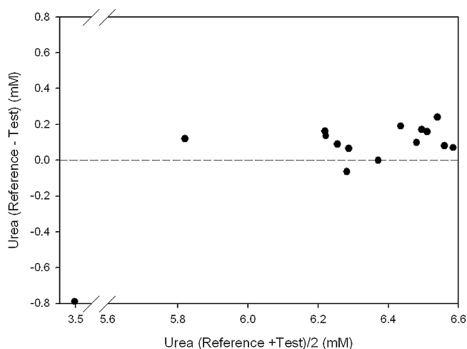
Fig. 5. Bland–Altman plot comparing the nanoPANI/urease biosensor (test) with the spectrophotometric assay (reference).
