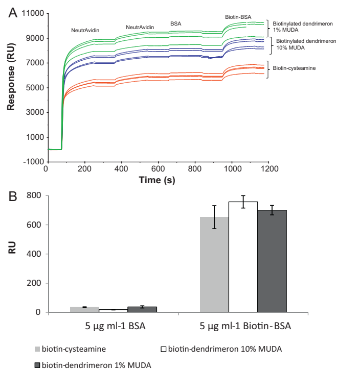
Fig. 2. (A) Sensorgram of the protein assay on NeutrAvidin captured surfaces; biotin-cysteamine, biotin-dendrimer on 1% MUDA and biotin-dendrimer on 10% MUDA surfaces. (B) Binding of BSA and biotinylated-BSA on NeutrAvidin immobilised on different biotinylated surfaces. A 5 \mu\text{g mL}^{-1} BSA and 5 \mu\text{g mL}^{-1} biotin-BSA were used.
