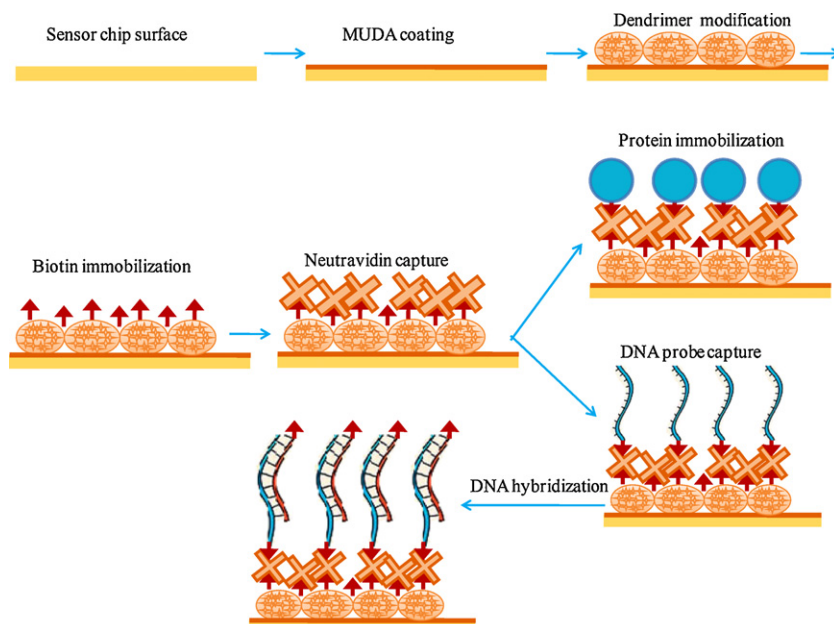
Scheme 2. Principle of the applied protein and DNA assays on the dendrimer modified MUDA-SAM.
