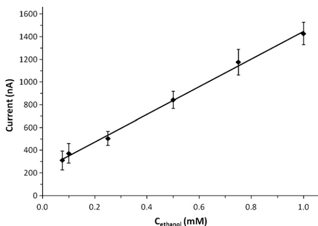
Fig. 5. Calibration plot using 9 sensors for each concentration: 3 prepared and used the same day, 3 stored 30 days at -20^\circ \text{C} and 3 stored 60 days at -20^\circ \text{C} .
