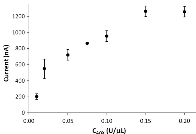
Fig. 3. Effect of the enzyme concentration on the responses for 1 mM ethanol of different biosensors prepared with SPCPEs and AOX from Hansenula . Data are given as average \pm SD ( n=3 ).
