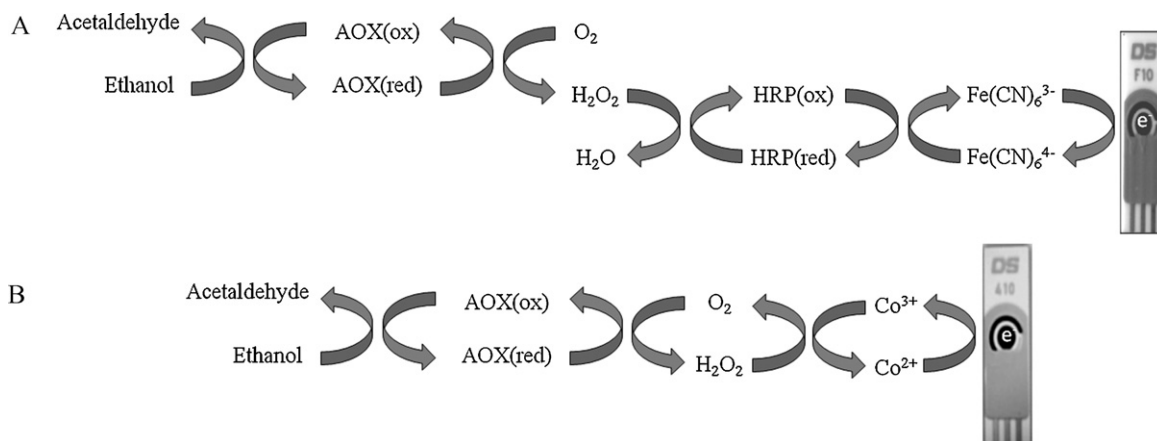
Fig. 1. Enzymatic reactions at the surface of SPPBCEs and SPCPCEs (A) and SPCPCEs (B).
