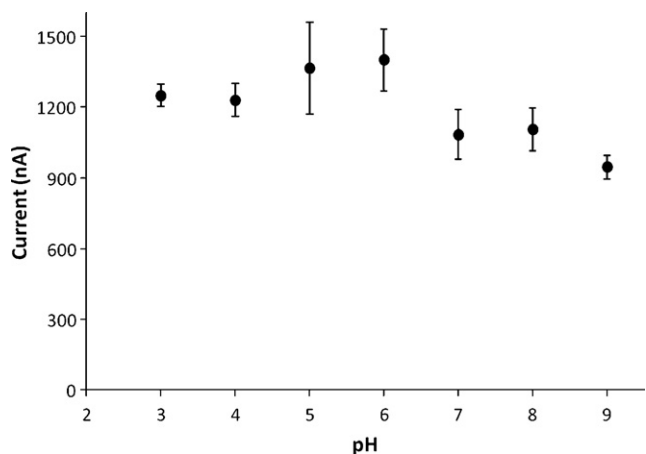
Fig. 4. Effect of the pH value on the response of the biosensor constructed with SPCPEs and AOX from Hansenula ( 0.15 \text{ U } \mu\text{L}^{-1} ). Ethanol concentration, 1 mM. Data are given as average \pm SD ( n=3 ).
