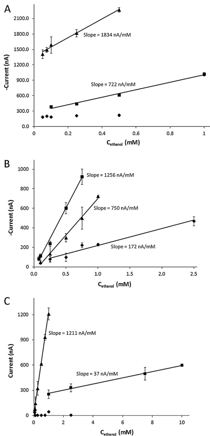
Fig. 2. Calibration plots for ethanol obtained with SPPBCEs (A), SPFCes (B) and SPCPCEs (C)-based biosensors. AOX from Hansenula ( \blacktriangle ), Pichia pastoris ( \blacksquare ) and Candida boidinii ( \blacklozenge ). Ethanol diluted in phosphate buffer 0.1 M pH 6. Data are given as average \pm SD ( n = 3 ).
