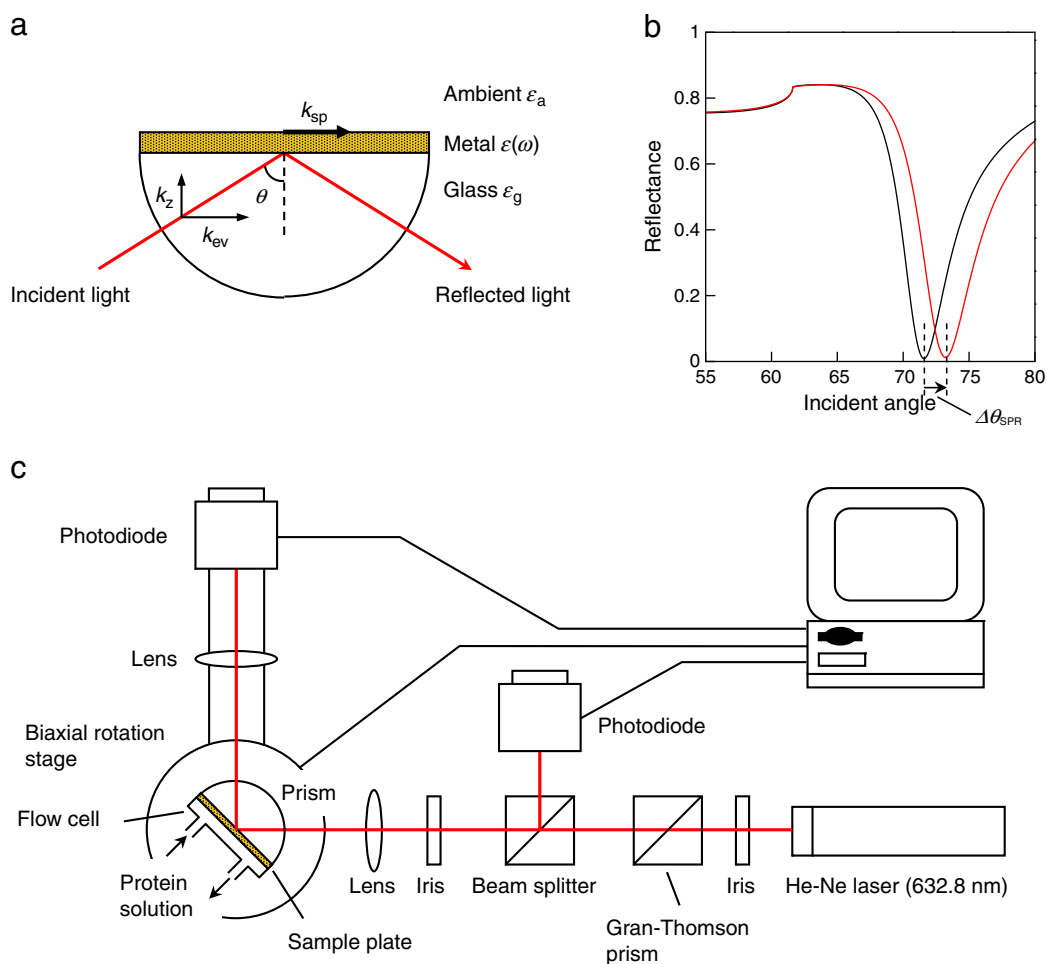
Fig. 1. (a) Schematic illustration of the Kretschmann configuration for SPR. Surface plasmon is excited at metal/ambient interface when the evanescent component of wave vector of incoming light ( k_{ev} ) is equal to the wave vector of the propagating surface plasmon ( k_{sp} ). (b) Reflectance as a function of incident angle before (black) and after (red) adsorption of substances. (c) Schematic representation of an SPR apparatus.
