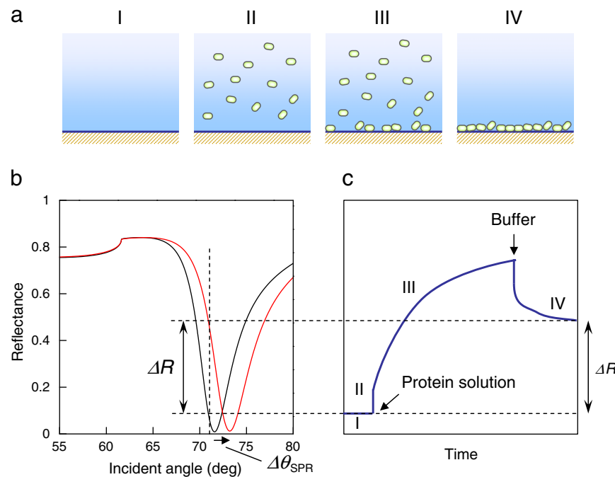
Fig. 2. Schematic illustration of an SPR profile during a protein adsorption experiment. (a) Sequential step in protein adsorption onto a material surface; surface exposed to buffer (I), upon exposure to protein solution (II), adsorbed with protein (III), and rinsed with buffer (IV). (b) Reflectance as a function of incident angle before (black) and after (red) adsorption of proteins. A shift in the SPR angle ( \Delta\theta_{\text{SPR}} ) occurs in a manner dependent on the amount of adsorbed proteins. (c) In real-time monitoring, reflectance at a specific incident angle (dashed line in (b)) is plotted as a function of time. Points I to IV correspond to steps in (a). Change in reflectance after protein adsorption ( \Delta R ) is finally converted to \Delta\theta_{\text{SPR}} to calculate the amount of adsorbed proteins.
