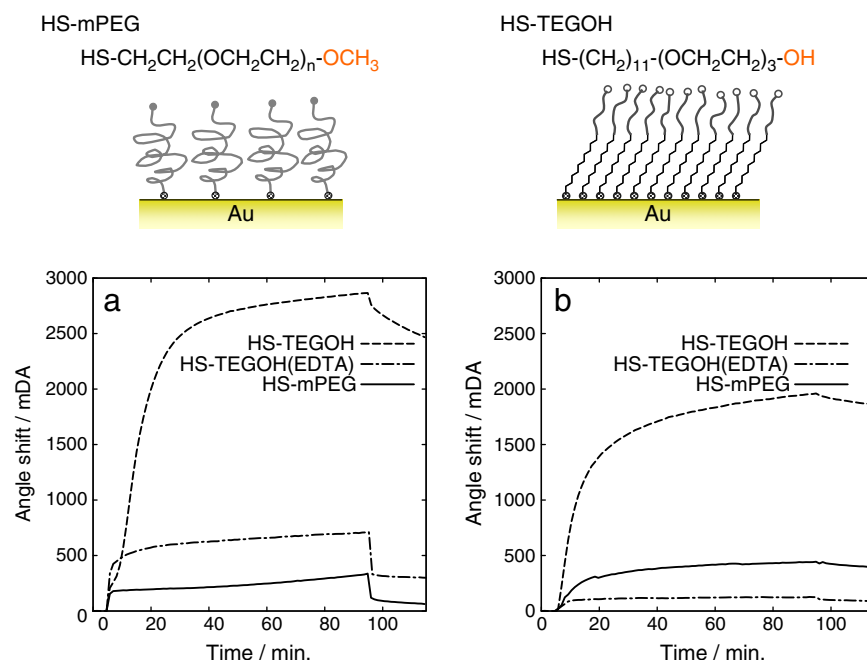
Fig. 9. SPR sensorgrams during exposure of HS-TEGOH and HS-mPEG surfaces to 10% human serum (a) and anti-C3b antiserum (b). Figures also include SPR sensorgrams when HS-TEGOH surface was exposed to 10% human serum in the presence of 10 mM EDTA to block the complement activation [90].
