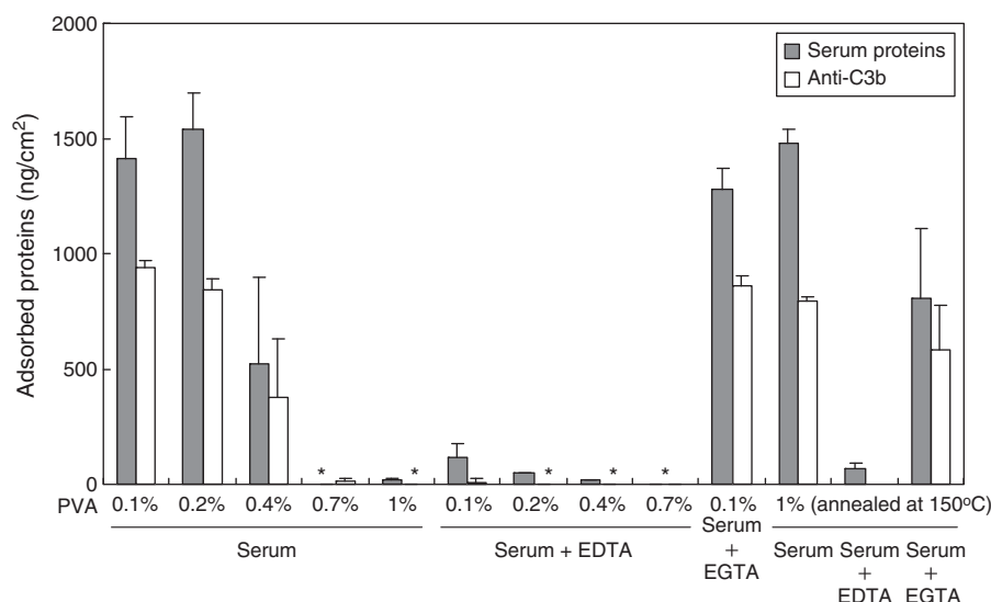
Fig. 10. Amounts of serum proteins adsorbed on PVA surfaces and subsequent binding of anti-C3b antibodies to serum protein layers formed on those surfaces. Data shown are means \pm SD ( n = 3 ). PVA percent: PVA concentration for spin-coating. Types of serum samples: serum, human serum; serum + EDTA, human serum + 10 mM EDTA; serum + EGTA, human serum + 10 mM EGTA + 2.5 mM MgCl_2 . Asterisks indicate that adsorption of serum proteins or binding of anti-C3b antibody was not detected by SPR [61].
