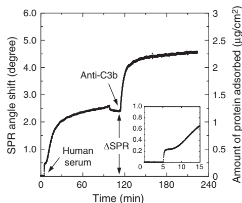
Fig. 5. Time curve of normal human serum proteins adsorption on OH-SAM and subsequent binding of anti-C3b antiserum. Modified from Ref. [67].
