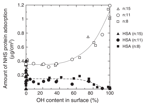
Fig. 8. The amounts of adsorbed serum proteins from 10% human serum (open symbols) and adsorbed human serum albumin (HSA) (closed symbols) from a single HSA solution as a function of hydroxyl density of mixed SAMs carrying hydroxyl and methyl groups. Mixed SAMs were formed from various reaction mixtures of 11-mercapto-1-undecanethiol and several methyl-terminated alkanethiols with different alkyl chain length (see Fig. 4). Modified from Ref. [54].
