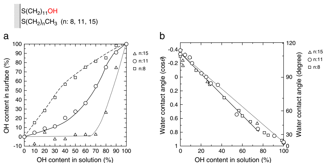
Fig. 4. Composition (a) and water contact angles (b) of SAMs formed from various reaction mixtures of 11-mercapto-1-undecanol and several methyl-terminated alkanethiols with different alkyl chain length. The composition of SAMs was determined by FTIR-RAS spectra. Modified from Ref. [54].
