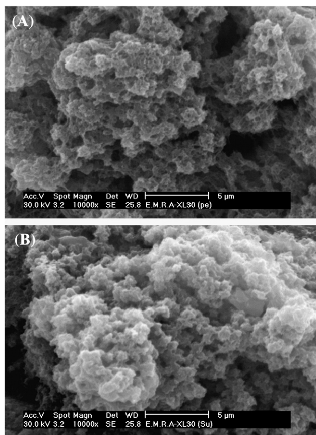
Fig. 9. SEM image of the PEDOT layers deposited on Pt wire from 0.01\text{ mol L}^{-1} EDOT in 0.1\text{ mol L}^{-1} \text{LiClO}_4 in acetonitrile (10 cycles) (magnification 10,000\times , 30\text{ kV} ), (A) in absence of SDS, (B) in presence of 150\text{ }\mu\text{L} 0.1\text{ mol L}^{-1} SDS.
