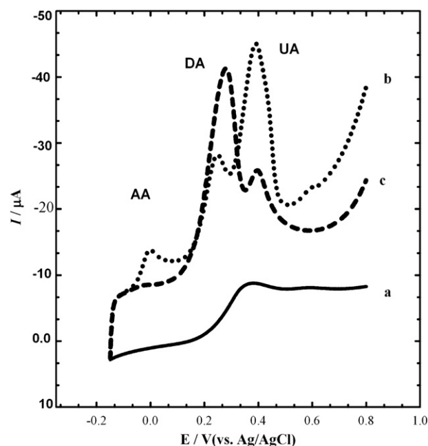
Fig. 6. LSVs for equimolar solution of 0.5 mmol L -1 AA, DA and UA in B-R (0.1 mol L -1 ) at pH 7.4, scan rate: 50 mV s -1 , at (a) bare Pt, (b) PEDOT/Pt and (c) PEDOT/Pt in presence of 150 \mu L of 0.1 mol L -1 SDS.
