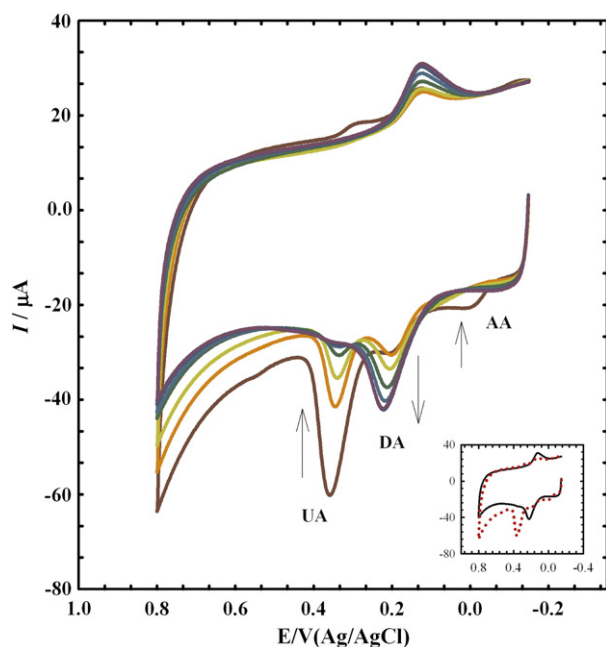
Fig. 7. Cyclic voltammogram for 0.2 \text{ mmol L}^{-1} AA, 0.1 \text{ mmol L}^{-1} UA and 0.1 \text{ mmol L}^{-1} DA in B-R ( 0.1 \text{ mol L}^{-1} ), at PEDOT/Pt with successive additions of ( 0 – 150 \mu\text{L} ) 0.1 \text{ mol L}^{-1} SDS, at \text{pH} 7.4 , inset represents the initial and final CVs.
