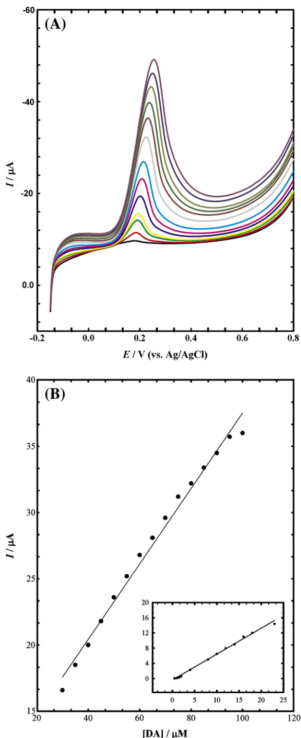
Fig. 3. (A) LSVs of 10 ml of 0.1 \text{ mol L}^{-1} B-R PH 7.4 at PEDOT/Pt electrode in 0.1 \text{ mol L}^{-1} 150 \mu\text{l} SDS in different concentrations of DA ( 0.5 \mu\text{mol L}^{-1} – 0.1 \text{ mmol L}^{-1} ) (B) calibration curve for DA for concentrations from ( 30 \mu\text{mol L}^{-1} to 0.1 \text{ mmol L}^{-1} ) and from ( 0.5 \mu\text{mol L}^{-1} to 25 \mu\text{mol L}^{-1} , the inset).
