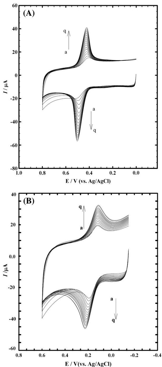
Fig. 1. Cyclic voltammograms of 5.0 \times 10^{-4} mol L ^{-1} dopamine/0.1 mol L ^{-1} B-R, scan rate 50 \text{ mV s}^{-1} at PEDOT/Pt electrode with successive additions ( 10 \mu\text{L} – 150 \mu\text{L} ) of 0.1 \text{ mol L}^{-1} SDS with stirring the solution for 5 min every addition and 1 min for occupation (a–q) at (A) pH 2.3 and (B) pH 7.4.
