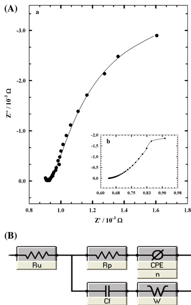
Fig. 8. Nyquist diagrams ( -Z'' vs. Z' ) for the EIS measurements at PEDOT / Pt (A) at potential 250 \text{ mV} . (a) In absence of SDS and (b) in presence of SDS (inset). In 5 \text{ mmol L}^{-1} DA in 0.1 \text{ mol L}^{-1} B-R \text{pH} = 7.4 . Amplitude: 5 \text{ mV} , frequency range: 0.1 – 100,000 \text{ Hz} (B) the equivalent circuit.
