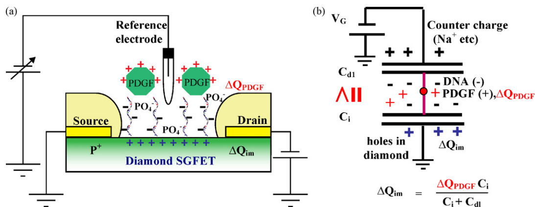
Fig. 1. (a) The static device characteristics of diamond SGFET by PDGF binding with aptamer and the mechanism of detecting signal depending on the surface-charge change. (b) C_i represents the surface capacitance of solid surface, C_{dl} represents the electric double-layer (liquid side) capacitance, \Delta Q_{im} represents a decreased carrier density by PDGF reaction with aptamer and \Delta Q_{PDGF} represents a decreased negative charge by PDGF reaction with aptamer.
