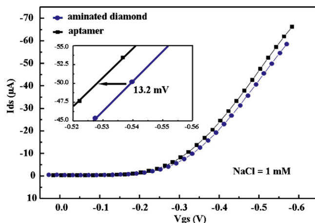
Fig. 2. The comparison of I_{ds} – V_{gs} characteristics between aminated and aptamer immobilization on diamond surface.
