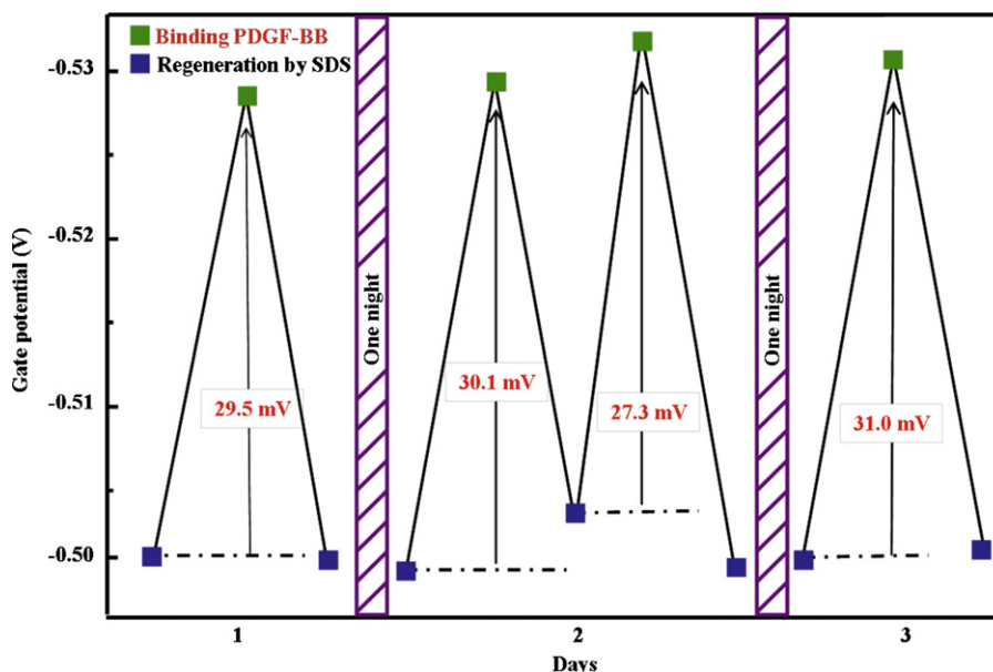
Fig. 4. Transfer characteristics of a SGFET over four cycles in PDGF binding to the aptamer and regeneration were performed repeatedly on functionalized diamond surfaces. The gate potential shift was observed at I_{ds} = -40 \mu A . The reproducible measurement yielded a SGFET is suitable for FET-type protein sensors.
