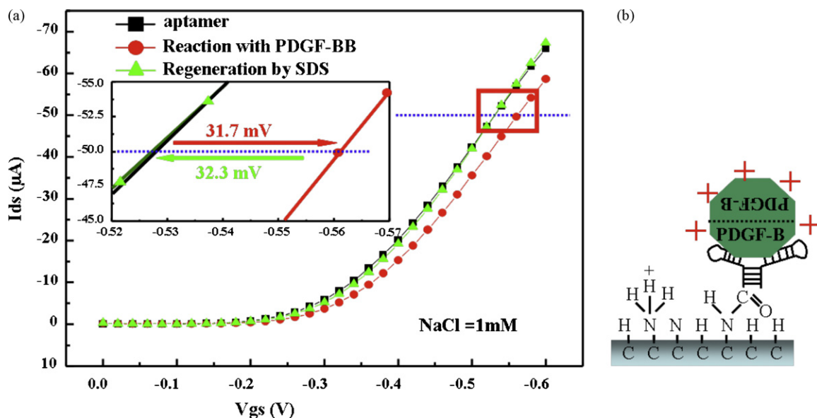
Fig. 3. (a) The directly exposed surface channel is very sensitive to surface charge on diamond SGFETs. After aptamer binding with PDGF on the functionalized surface channel, the surface negative charge decrease and hole carrier density also will decrease due to the decreased negative charge on the surface channel. With the introduction of PDGF, a 31.7 mV shift in the negative direction was observed. After the removal of PDGF (regeneration) by SDS, the voltage shift was 32.3 mV in the positive direction. (b) The schematic showing the procedure for detecting PDGF-BB on functionalized diamond surfaces by potentiometric method.
