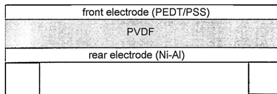
Fig. 6. A free standing, self-absorbing 28 \mu\text{m} PVDF pyroelectric sensor (Source: Setiadi et al., 1999a,b).
