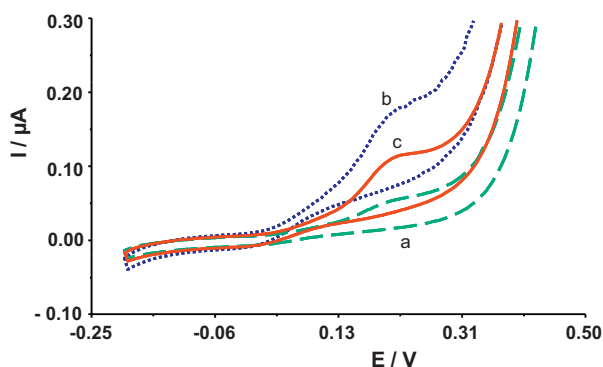
Fig. 2. CV obtained with a DNA-CPE at 50 \text{ mV s}^{-1} in tris-HCl buffer pH 9.0 in 0.5 \text{ mmol L}^{-1} NADH with 0.01 \text{ mol L}^{-1} \text{CaCl}_2 after: (a) immersion in Fenton solution and electrochemical oxidation (b) only electrochemical oxidation; (c) immersion in Fenton solution with 10 \mu\text{mol L}^{-1} AA and electrochemical oxidation.
