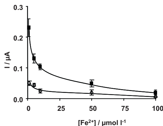
Fig. 3. Influence of \text{Fe}^{2+} concentration (ratio \text{Fe}:\text{EDTA}:\text{H}_2\text{O}_2 ; 1:2:40) on the electrocatalytic current intensity of 0.5 \text{ mmol L}^{-1} NADH with 0.01 \text{ mol L}^{-1} \text{CaCl}_2 in tris-HCl buffer at pH 9.0.
