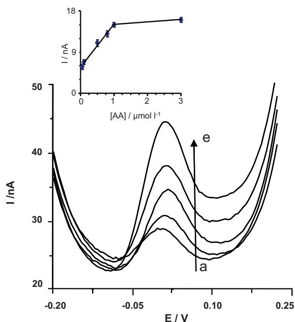
Fig. 4. DPVs obtained after immersion of DNA-CPE in Fenton solution containing a standard solution of AA: (a) 0.05, (b) 0.10, (c) 0.50, (d) 0.80 and (e) 1.00 \mu\text{mol L}^{-1} . Inset: relationship between I_a and AA concentration.
