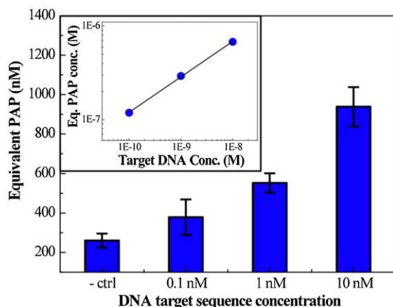
Fig. 5. A monotonic increase of generated PAP is found as target DNA concentration increases from zero to 1.0 \times 10^{-8} M. A significant difference is found between control and 1.0 \times 10^{-10} M chips ( P=0.05 ). Error bars are the standard deviation of 3 parallel measurements. Oxidation current is converted into equivalent PAP concentration using zero and 1.0 \times 10^{-6} M PAP as calibration points. Inset: On log–log scale (axes are same as the big plot), equivalent PAP concentration shows a linear dependence on target DNA for concentrations between 1.0 \times 10^{-10} and 1.0 \times 10^{-8} M.
