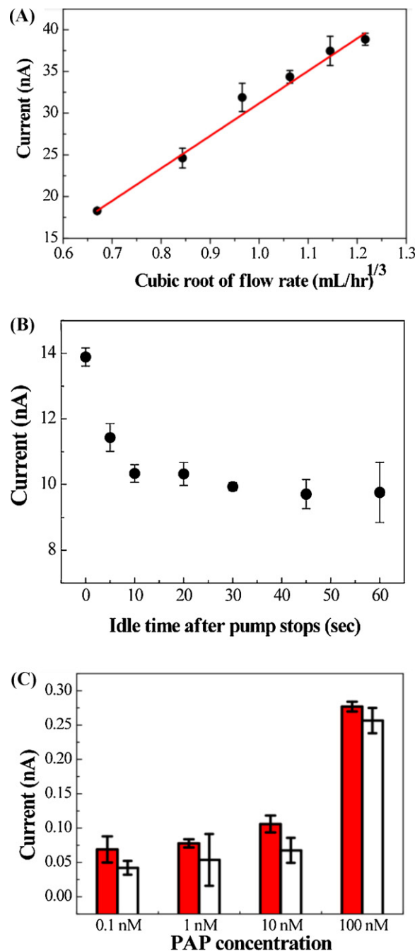
Fig. 2. (A) Flow rate effect on the measured current. Sample containing 1.0 \times 10^{-3} M PAP is purged into the microchannel at different flow rates between 0.3 and 1.8 mL/h by a syringe pump. The correlation follows the cubic root of the flow rate with correlation coefficient of 0.984 (mean \pm \sigma , n=3 ). (B) Impact of idle time on measured current after pump is stopped. Sample is pumped at 1.2 mL/h for 30 s. After 0, 5, 10, 20, 30, 45 or 60 s, oxidation current is collected for 10 s (mean \pm \sigma , n=3 ). (C) Comparison of measured current at different PAP concentration with (solid bars) or without (open bars) regeneration of electrode by flushing ethanol in between measurements (mean \pm \sigma , n=3 ).
