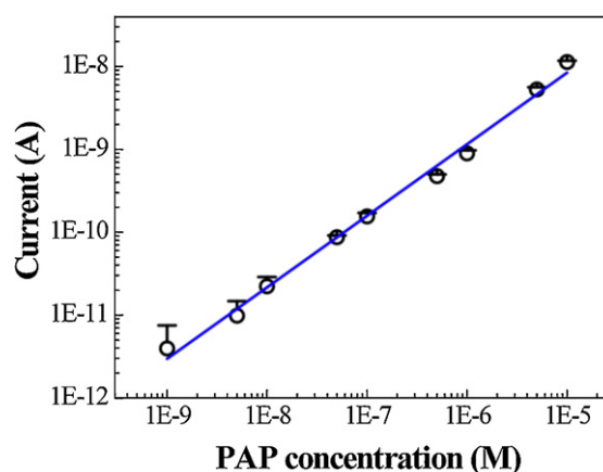
Fig. 3. Oxidation current vs. PAP concentration on log-log scale. A 15 \mu L sample was delivered into the microchannel with a syringe pump. The detection limit is 1.0 \times 10^{-10} M. The dynamic range is between 1.0 \times 10^{-9} M and 1.0 \times 10^{-5} M with a correlation coefficient of 0.994. The points represent the average value of 3 parallel measurements of the average current recorded between 9.75 and 10 s (mean + \sigma , n=3 ).
