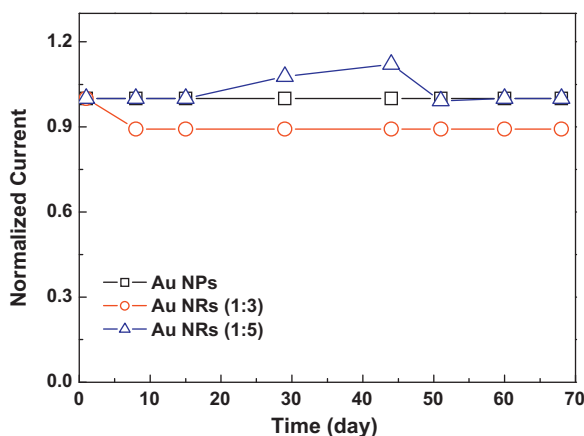
Fig. 6. Stability test of Au nanocrystal-based enzyme-free biosensors over 68 days in the PBS (0.05 M, pH 5) containing 10 mM [Fe(CN) 6 ] 3-/4- at 200 mV to 0.33 mM hydrogen peroxide.
