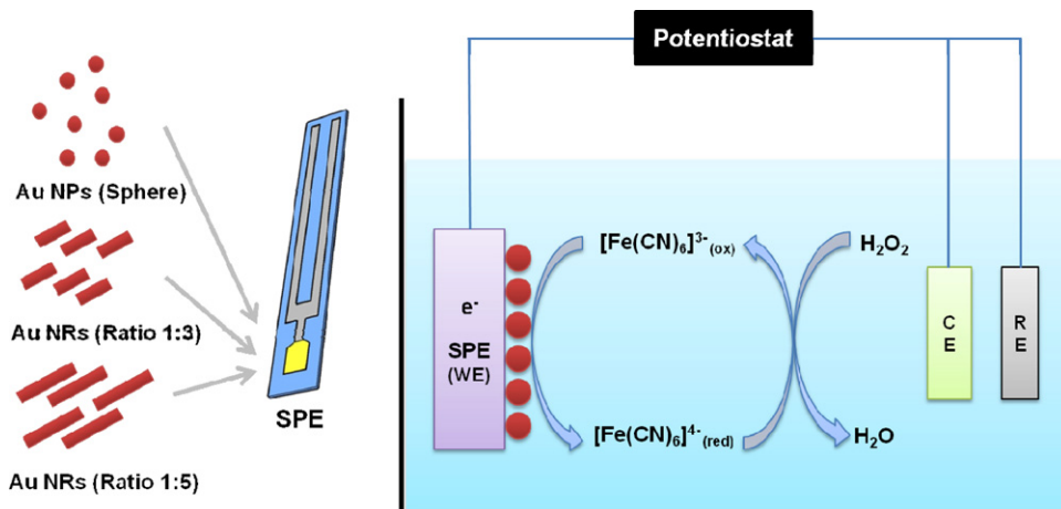
Fig. 2. Schematic of enzyme-free hydrogen peroxide biosensor and the reaction on the electrode (SPE: screen printed electrode, WE: working electrode, CE: counter electrode, RE: reference electrode).
