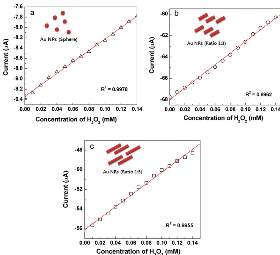
Fig. 5. Amperometric responses of enzyme-free biosensors for the detection of hydrogen peroxide in PBS (0.05 M, pH 5) containing 10 mM [Fe(CN) 6 ] 3-/4- at an applied potential of 200 mV with successive additions of 0.01 mM hydrogen peroxide. (a) Au NS-based, (b) Au NR (1:3)-based, and (c) Au NR (1:5)-based biosensors, separately.
