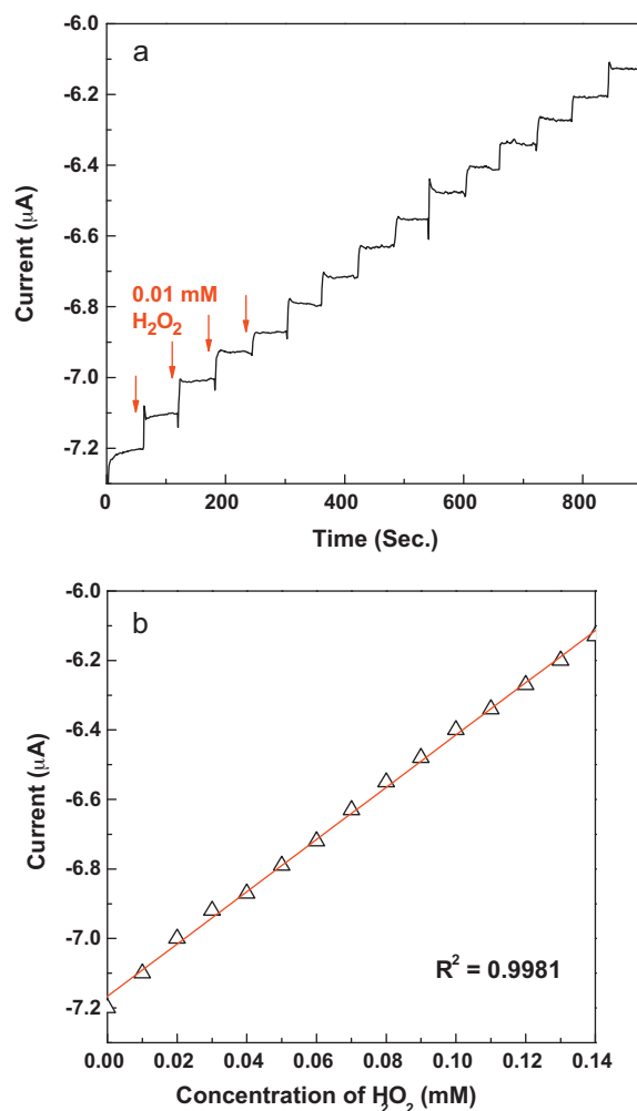
Fig. 4. Amperometric response of Au NS-based enzyme-free biosensors for the detection of hydrogen peroxide (a) response in PBS (0.05 M, pH 5) containing 5 mM [\text{Fe}(\text{CN})_6]^{3-/4-} at an applied potential of 200 mV with successive additions of 0.01 mM hydrogen peroxide (b) calibration plot (current vs. concentration of hydrogen peroxide) with linear regression analysis.
