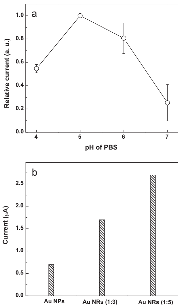
Fig. 3. Amperometric responses of (a) the biosensor with Au NSs to various pH values of PBS (0.05 M) containing 10 mM [\text{Fe}(\text{CN})_6]^{3-/4-} at 200 mV to 0.33 mM hydrogen peroxide, (b) the biosensors with Au NSs, Au NRs (1:3), and Au NRs (1:5) in the PBS (0.05 M, pH 5) containing 10 mM [\text{Fe}(\text{CN})_6]^{3-/4-} at 200 mV to 0.33 mM hydrogen peroxide.
