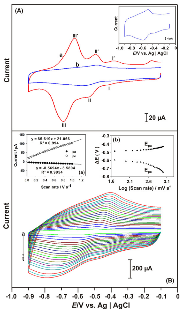
Fig. 3. (A) CVs of (a) CACNT and (b) CAT/CACNT film modified GCEs obtained at the scan rate of 50 mV s -1 . Inset is the enlarged view of (b). (B) CVs obtained at CAT/CACNT/GCE at different scan rates. Scan rates from (a–t) are 50, 100, 150, 200, 250, 300, 350, 400, 450, 500, 550, 600, 650, 700, 750, 800, 850, 900, 950 and 1000 mV s -1 respectively. Supporting electrolyte: N 2 saturated PBS. The inset plots are (a) the peak currents ( I_{pa} and I_{pc} ) vs. scan rate/V s -1 and (b) variation of peak potential vs. log (scan rates).
