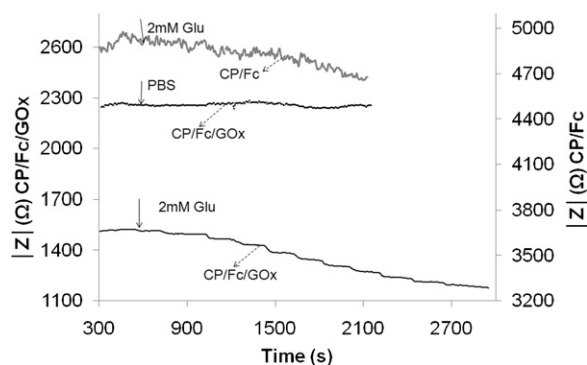
Fig. 1. On-line response of the biosensor and controls: (—) CP/Fc/GOX biosensor; (---) CP/Fc without GOx both with the addition of glucose; and (...) biosensor with the addition of support electrolyte (PBS) without glucose.
