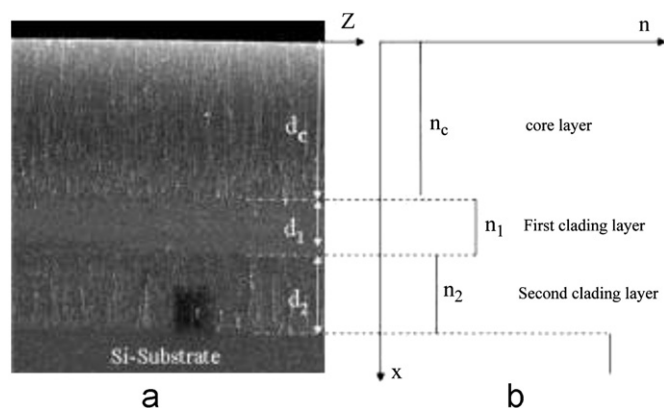
Fig. 1. SEM cross section image of the porous silica ARROW structure (a) and refractive index profile (b).
