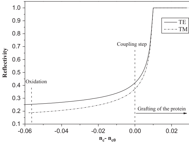
Fig. 3. Calculated reflectivity as a function of the refractive index variation of the core layer after each step (functionalization and BSA grafting), with constant values of n_1 and n_2 for TE and TM modes, working wavelength \lambda = 1.55 \mu\text{m} , d_c = 3.8 \mu\text{m} and d_1 = 1.4 \mu\text{m} .
