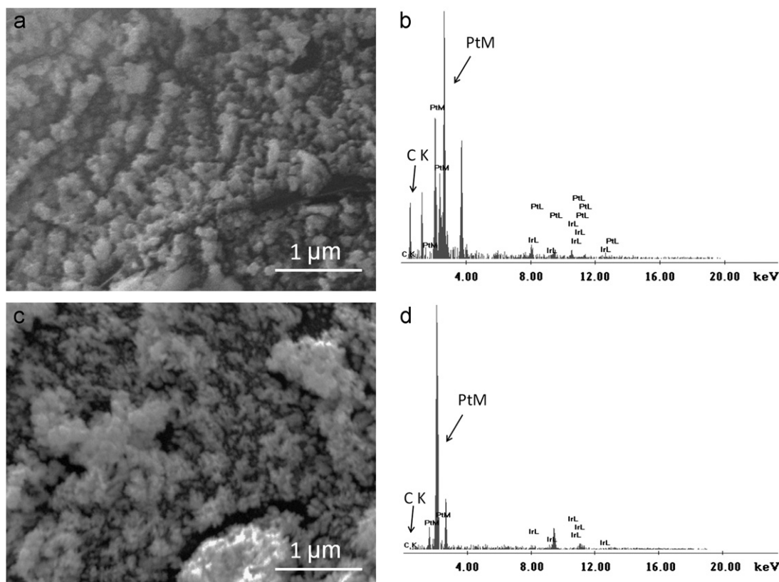
Fig. 1. Representative SEM image and EDS spectrum of GrO x /Pt-black microelectrode ((a) and (b), respectively) and Pt-black microelectrode ((c) and (d), respectively). In EDS, the peak for carbon was noted as "C K" and for platinum as "Pt M" ("K" and "M" represent the electron shells).
