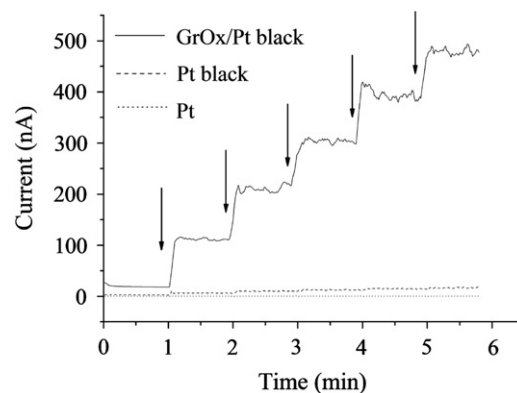
Fig. 3. Representative amperometric response to H 2 O 2 for unmodified, Pt-black and GrO x /Pt-black microelectrodes at +500 mV (arrows indicate addition of 10 μM H 2 O 2 ).
