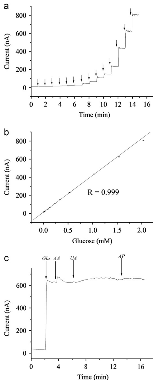
Fig. 5. (a) Representative amperometric response to glucose in the whole linear range (1 \mu\text{M} – 2 mM) for \text{GrO}_x/\text{Pt-black} microbiosensors at +500 mV (arrows (from left to right) indicate addition of 1, 1, 5, 10, 10, 50, 50, 100, 100, 200, 500, and 500 \mu\text{M} glucose). (b) Linear regression for (a) (error bars represent standard error of the mean). (c) Representative amperometric response to 2 mM glucose (noted as "Glu"), 125 \mu\text{M} ascorbic acid (AA), 330 \mu\text{M} uric acid (UA), and 130 \mu\text{M} acetaminophen (AP) for \text{GrO}_x/\text{Pt-black} microbiosensors.
