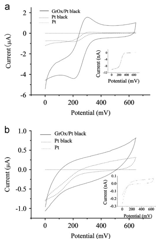
Fig. 2. Representative CV of unmodified Pt, Pt-black and GrO x /Pt-black microelectrodes at +20 mV/s in (a) 4 mM Fe(CN) 6 3- /1 M KNO 3 and (b) 0.01 M PBS. Insets: CV for the unmodified microelectrode.
