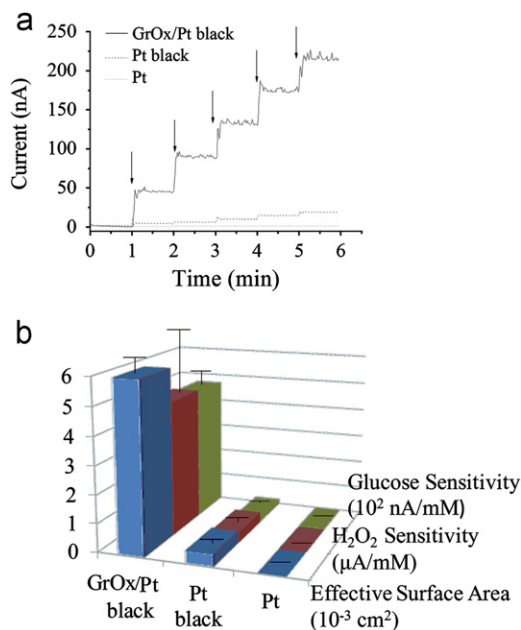
Fig. 4. (a) Representative amperometric response of glucose microbiosensors based on unmodified, Pt-black and \text{GrO}_x/\text{Pt-black} microelectrodes at +500 mV (arrows indicate addition of 100 \mu\text{M} glucose). (b) Histogram showing the major electrochemical parameters of unmodified Pt, Pt-black and \text{GrO}_x/\text{Pt-black} microelectrodes (error bars represent standard error of the mean).
