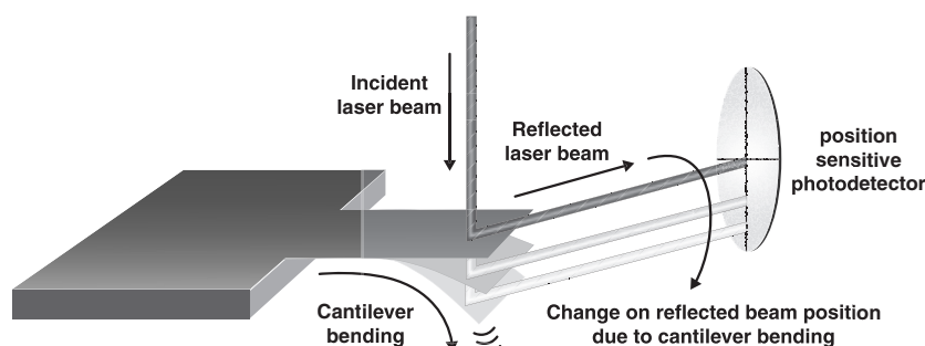
Fig. 1. Scheme of the optical read-out method to monitor cantilever bending. Reprinted from Ref. [32] with permission from Elsevier.
