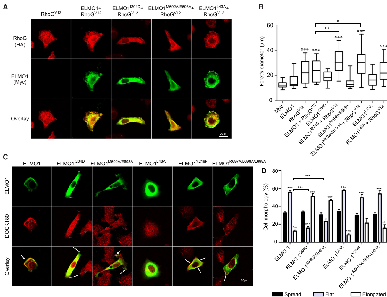
Figure 4. The EID/EAD Intramolecular Interaction Is a Regulatory Feature of ELMO in Cells
