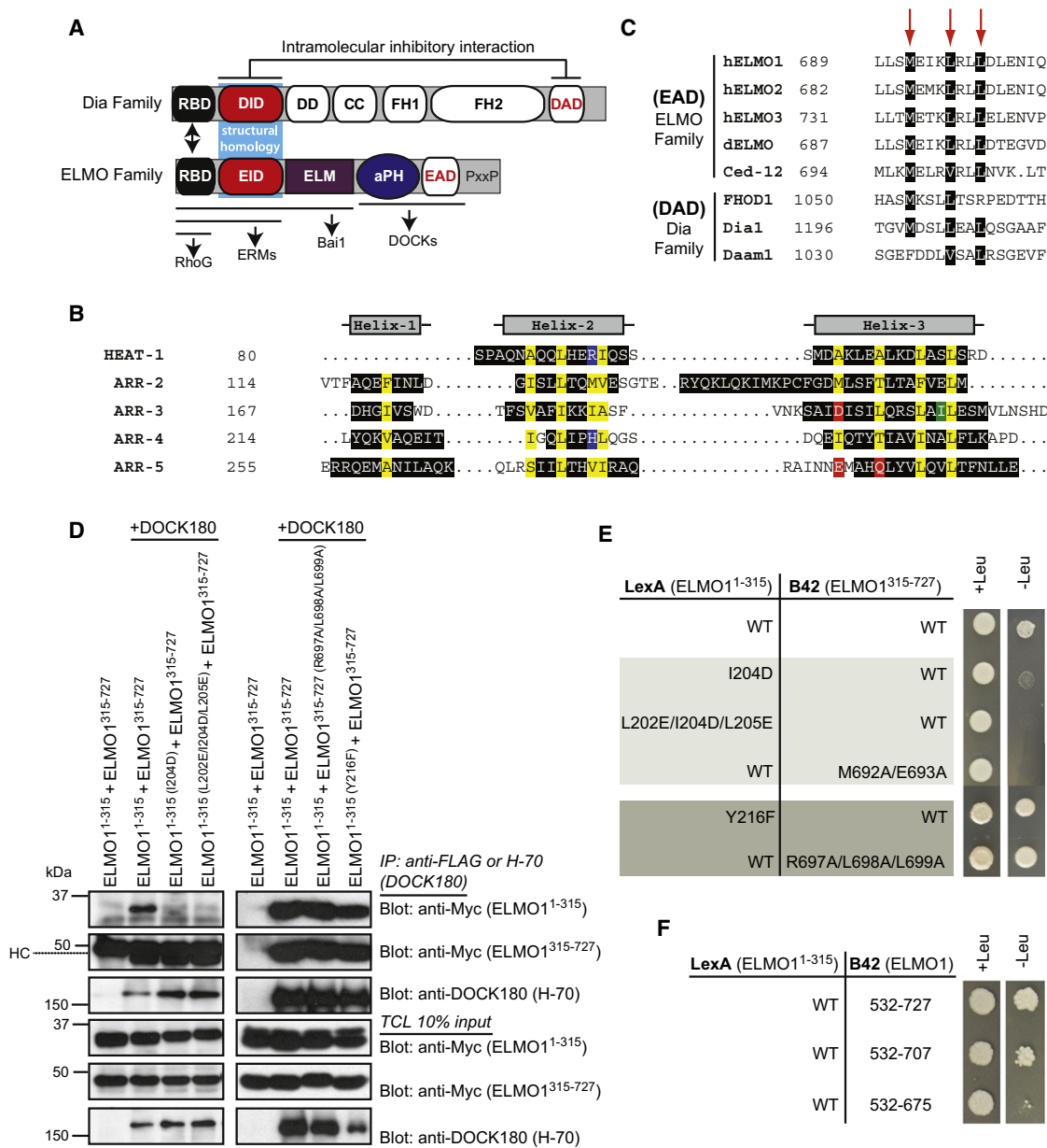
Figure 1. Intramolecular Interactions in ELMO1 through Novel Domains
