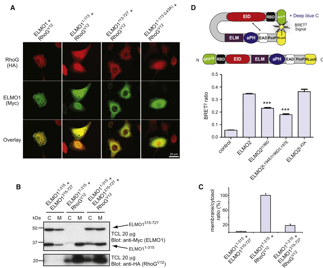
Figure 3. Full-Length ELMO2 Is Autoinhibited and Regulated by RhoG Binding to the RBD
