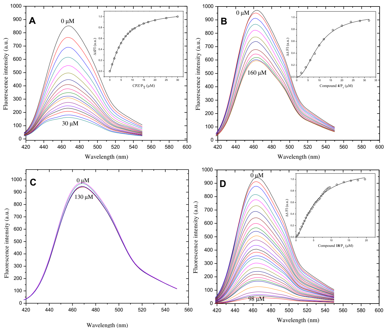
Fig. 1. Fluorescence spectra and titration curves of \text{Ca}^{2+} -hCaM-M124C-mBBr in the presence of CPZ (A), 4 (B), 11 (C), and 18 (D). Buffer was 100 mM of potassium acetate (pH 5.1) at 37 °C and 1 mM \text{CaCl}_2 . Samples were excited at 381 nm, and emission spectra recorded for light scattering effects from 400 to 550 nm. The absolute changes of maximal fluorescence emission were plotted against the ration compounds/protein total and fitted to the binding equation model to obtain the K_m .
