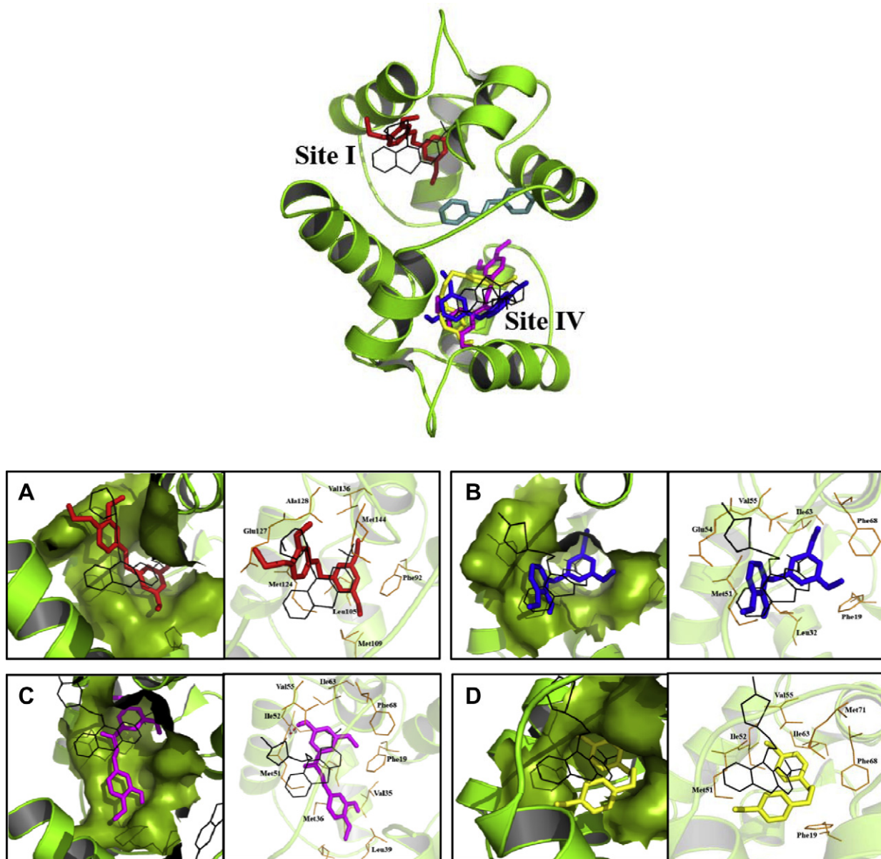
Fig. 2. Binding model of compounds with the complex \text{Ca}^{2+} -CaM. CaM is represented in green cartoon. The TFP is depicted in black lines, compound 4 in red sticks, 11 in cyan sticks, 13 in blue sticks, 17 in magenta sticks and 20 in yellow stick. Hydrophobic pockets are shown in surface and interacting amino acids within the CaM-ligands complex of the compounds 4 (A), 13 (B), 17 (C) and 20 (D). This figure was generated using the program PyMOL. (For interpretation of the references to color in this figure legend, the reader is referred to the web version of this article.)
