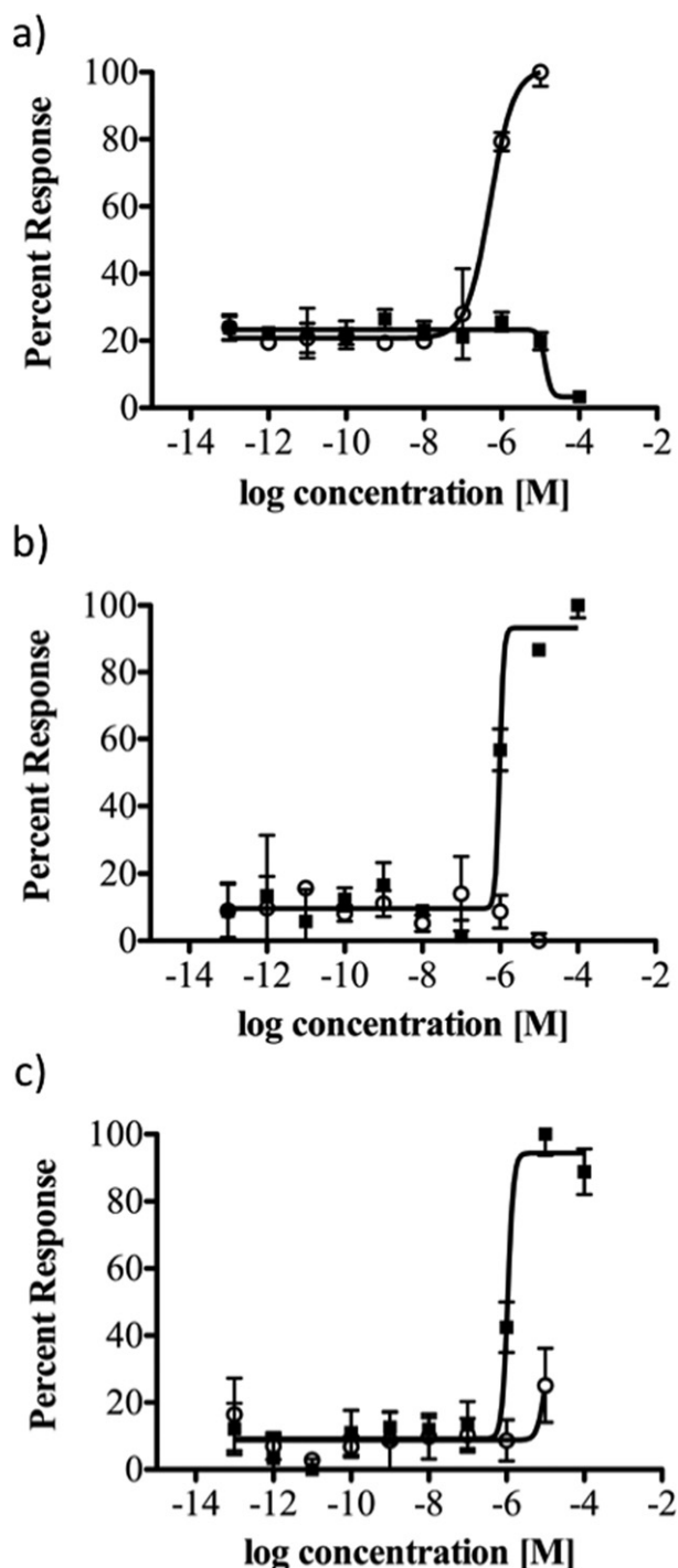
Fig. 4. The effect of 17- \beta -estradiol ( E_2 ; white circles) and 3,5,3'-triiodo-L-thyronine ( T_3 ; black squares) on E. coli D1210 \Delta thyA cells transformed with (A) pMIT::ER \beta , (B) pMIT::TR \alpha and (C) pMIT::TR \beta . The experiments were performed in -Thy medium at 34 °C. Experiments were carried out in triplicate, and optical densities at 600 nm were recorded after 24 h. Error bars represent one standard deviation from the mean for each ligand concentration.
