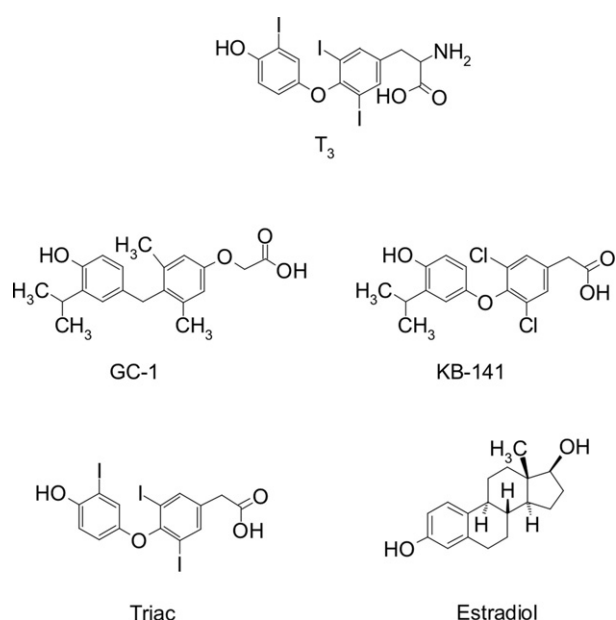
Fig. 1. Structures included in the study: T 3 [CAS: 6893–02–3]; Triac [CAS: 51–24–1]; KB-141 [CAS: 219691–94–8]; GC-1 [CAS: 211110–63–3]; 17-β-estradiol (E 2 ) [CAS: 50–28–2].
