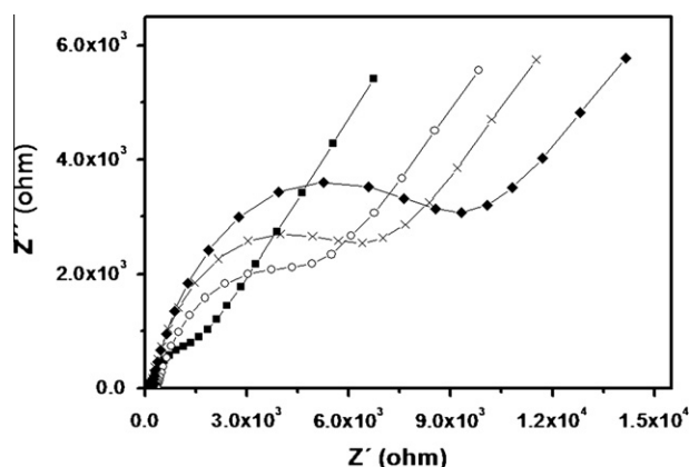
Fig. 3. Nyquist plots for the stepwise modification process: bare gold electrode (■), AuNP/PANI (○), AuNP/PANI-BmoLL (×) and AuNP/PANI-BmoLL-BSA (◆). Supporting electrolyte 10 \text{ mM } \text{K}_4[\text{Fe}(\text{CN})_6]/\text{K}_3[\text{Fe}(\text{CN})_6] 1:1 containing 0.15 \text{ M} NaCl in PBS solution pH 7.4.
