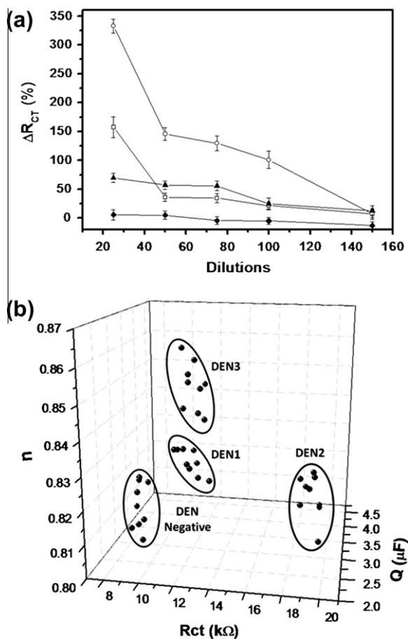
Fig. 6. \Delta R_{CT} for the systems that corresponded to the AuNPANI-BmoLL-BSA-DEN1 ( \square ), AuNPANI-BmoLL-BSA-DEN2 ( \circ ), AuNPANI-BmoLL-BSA-DEN3 ( \blacktriangle ) and AuNPANI-BmoLL-BSA-DENnegative ( \blacklozenge ) at different concentrations (1:25, 1:50, 1:75, 1:100 and 1:150) (a); and three-dimensional plot for values of R_{CT} , Q and n (b). The analyses of the sera of patients contaminated with dengue (three patients for each serotype) and serum control (three patients) were performed in triplicate.
