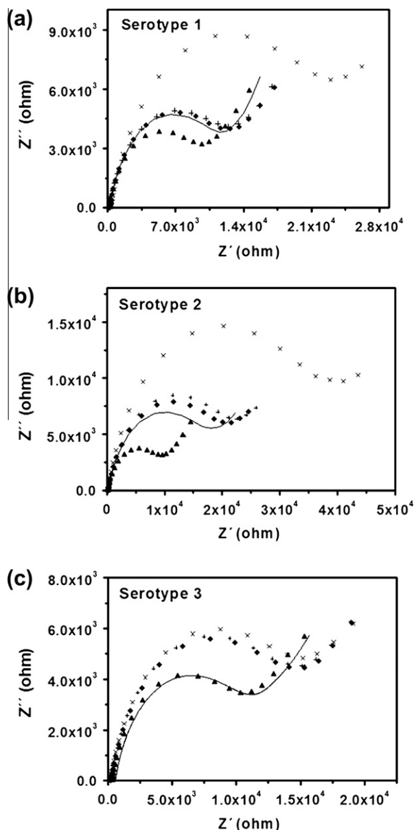
Fig. 4. Nyquist plots of AuNPANI-BmoLL-BSA response after contact with DEN1 (a), DEN2 (b) and DEN3 (c) as follow: AuNPsPANI-BmoLL-BSA-DEN (1:150) (▲), AuNPsPANI-BmoLL-BSA-DEN (1:100) (●), AuNPsPANI-BmoLL-BSA-DEN (1:75) (◆), AuNPsPANI-BmoLL-BSA-DEN (1:50) (+), AuNPsPANI-BmoLL-BSA-DEN (1:25) (×). Supporting electrolyte 10 mM K_4[Fe(CN)_6]/K_3[Fe(CN)_6] 1:1 containing 0.15 M NaCl in PBS solution pH 7.4.
