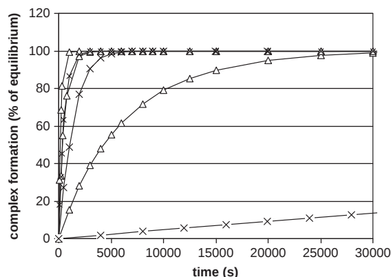
Fig. 1. Approach to equilibrium for complex formation in solution ( \Delta ) and at a chip surface (x). In both cases, the upper curve is for low-affinity, the middle curve is for intermediate affinity and the lower curve is for high affinity (see text).
