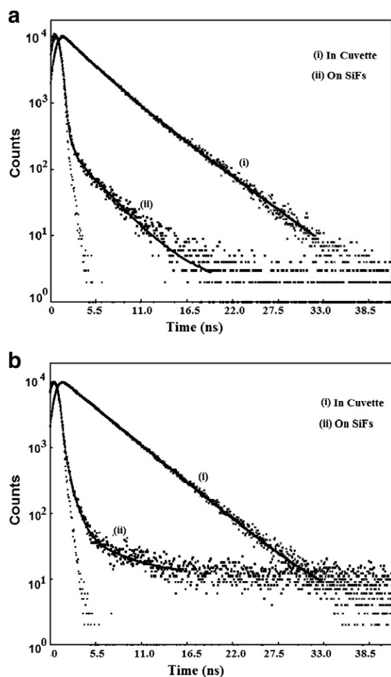
Fig. 4. Intensity decay profile of (a) Alexa 488 and (b) Alexa 594 on glass, a SiFs sandwich and in solution (cuvette) \lambda_{\text{ex}} = 467 nm.
