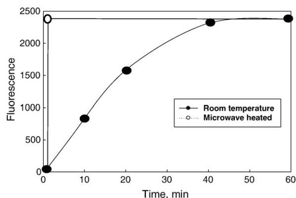
Fig. 2. Room temperature real-time hybridization kinetics for Alexa 594 nm and microwave acceleration for 30 s. The “Rapid Catch and Signal” assay is complete in less than 30 s.
