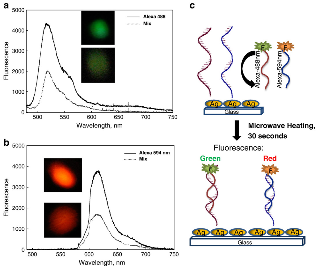
Fig. 3. (a) Emission spectra of Alexa 488 and a 1/1 mixture of both Alexa 488 and 594 dyes attached to a DNA/SiF film. Excitation was undertaken with a 473 nm laser line. (b) Emission spectra of Alexa 594 and a 1/1 mixture of both Alexa 488 and 594 dyes attached to a DNA/SiF film. Excited with a 594 nm laser line. (c) General scheme of 2-color DNA assay.
