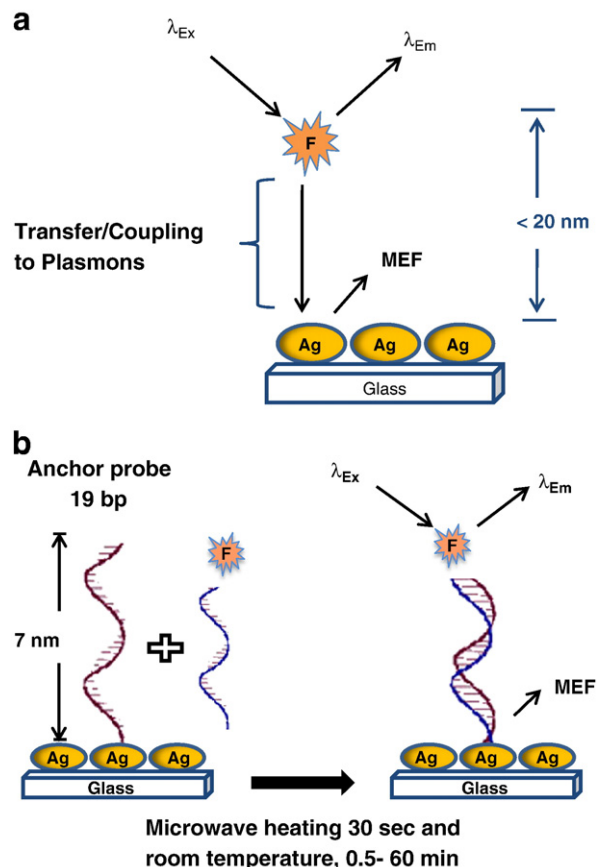
Fig. 1. (a) Graphical representation of the current interpretation of MEF. (b) MAMEF surface DNA capture assay, annealing in microwave cavity and the control assay run at room temperature, "Rapid Catch and Signal" technology.
