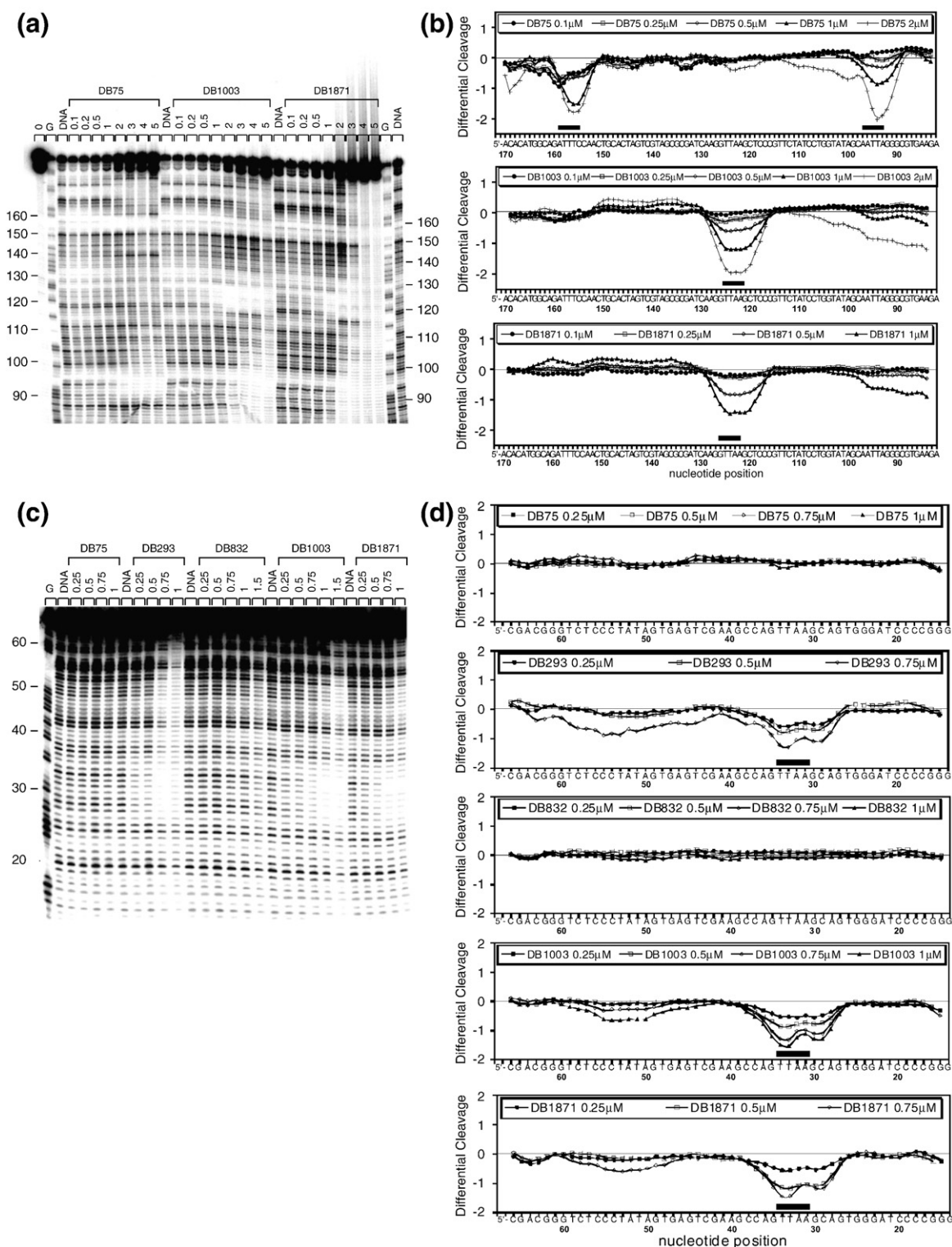
Fig. 7. DNase I footprinting assays. (a) The radiolabeled MS1-198 bp (lanes "DNA") or (c) TTA-69 bp DNA fragments were incubated alone (lanes "DNA") or in the presence of graded concentrations (in micromolar) of the various compounds as indicated on the top of each lanes. Lanes "G" correspond to the G-track ladders that were used as markers for guanines positions to locate the protected sites. The respective densitometric analyses are presented in (b) and (d). Black boxes localize the sites that are protected by the compounds from DNase I cleavage.
