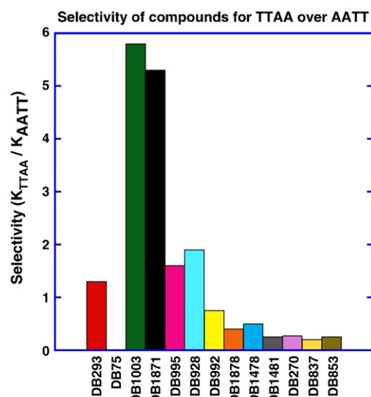
Fig. 9. Comparative plot of selectivity ( K_{TTAA}/K_{AATT} ) of studied compounds against AATT and TTAA sequences. K_{TTAA} = (\sqrt{K_1 \times K_2}) ; K_{AATT} is the equilibrium binding constant for the AATT site.
