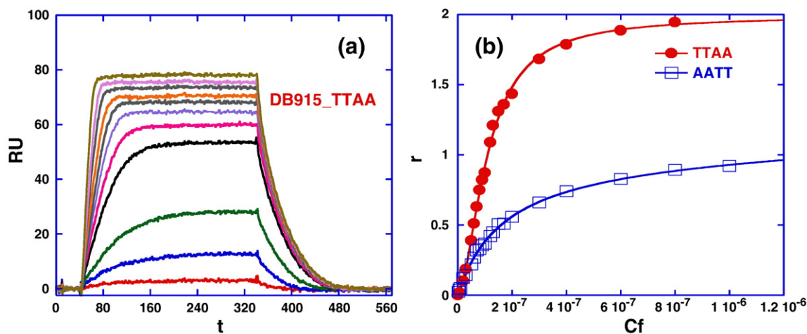
Fig. 5. Equilibrium binding studies. SPR sensorgrams for binding of (a) DB915 to the TTAA. The unbound compound concentrations in the flow solutions range from 0.0001 \mu M in the lowest curve to 0.8 \mu M in the top curve. (b) The binding plot for DB915 in the presence of TTAA and AATT.
