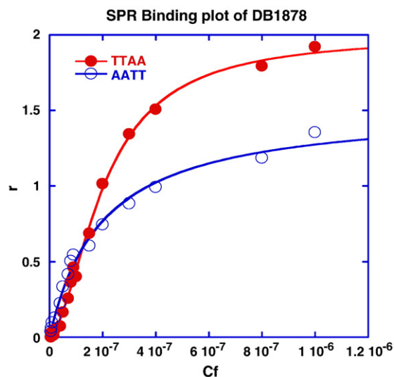
Fig. 8. Equilibrium binding studies. SPR binding plots for DB1878 in the presence of TTAA and AATT.
