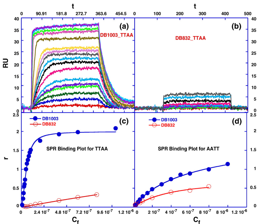
Fig. 4. Equilibrium binding studies. SPR sensorgrams for binding of (a) DB1003 and (b) DB832 to TTAA at 25 °C. The unbound compound concentrations in the flow solutions range from 0.0001 \mu M in the lowest curve to 0.8 \mu M in the top curve. The RU values from the steady-state region of SPR sensorgrams were converted to r by r = RU/RU_{max} and are plotted versus the unbound compound concentration for DB1003 and DB832 binding to (c) TTAA and (d) AATT.
