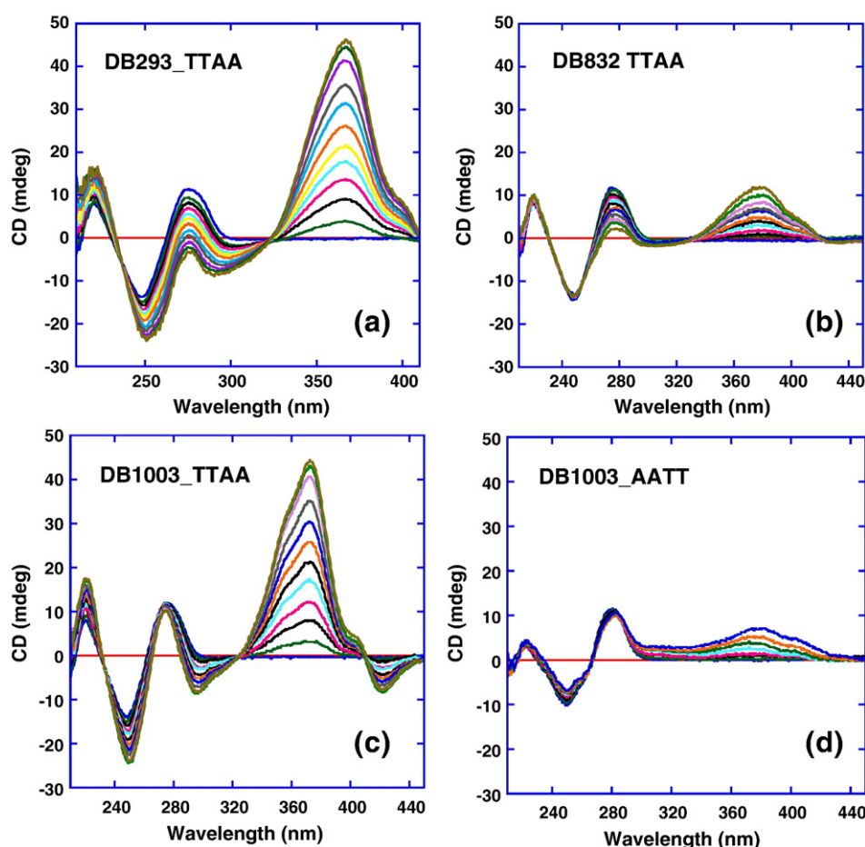
Fig. 3. Study of binding mode. CD titration for TTAA in (a) DB293, (b) DB832, (c) DB1003, and AATT in (d) DB1003. The concentration of duplex hairpin was 5 μM and the compound was added with 1 μM increment with a total of 10 increments. In case of DB293 and DB1003 in TTAA, DNA saturates at 2:1 compound-to-DNA ratio confirming dimer formation for these compounds. DB832 in TTAA and DB1003 in AATT with a similar compound-to-DNA ratio give weaker binding.
