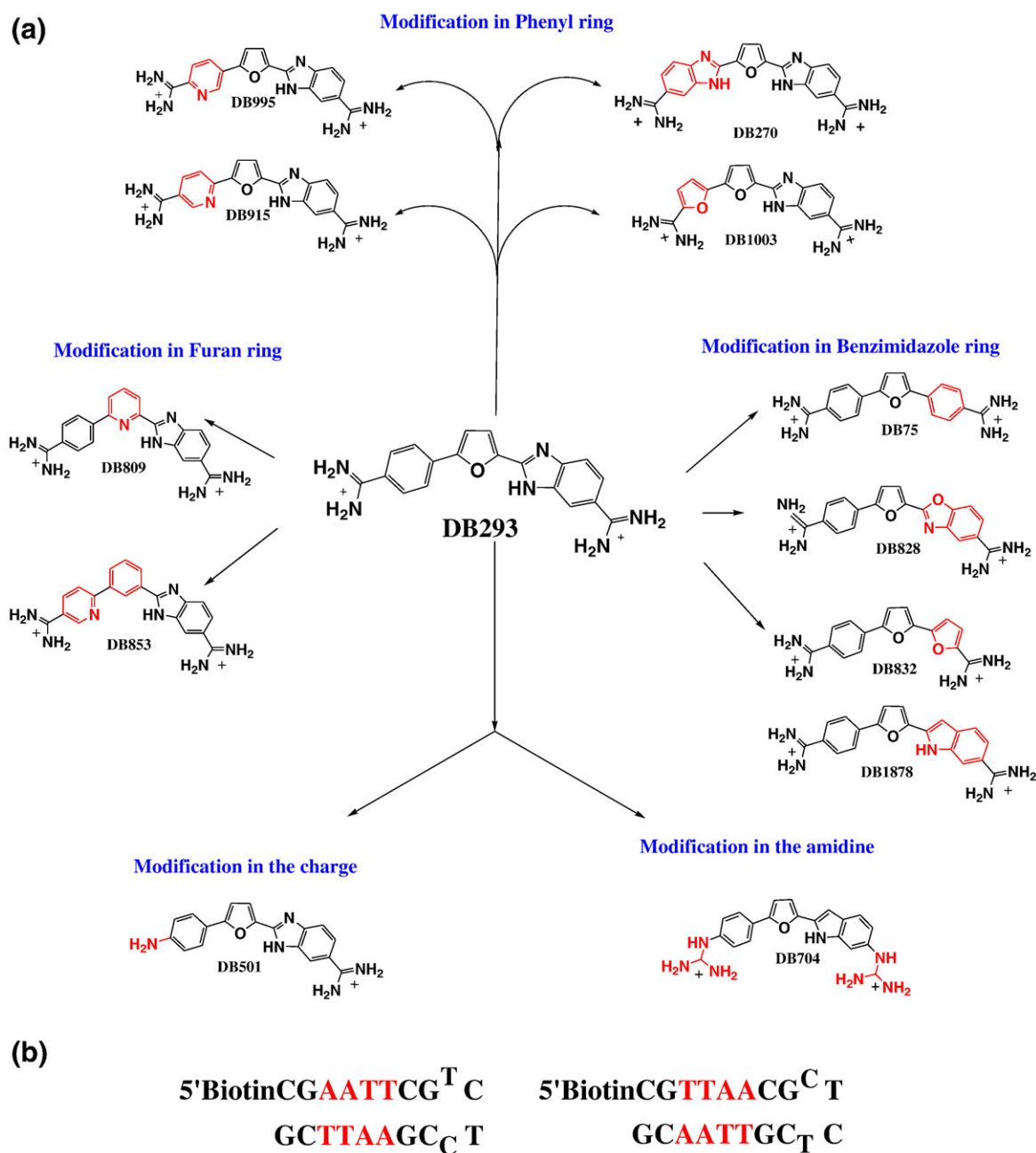
Fig. 1. (a) Representative structures of compounds classified by their functional group modifications. Structures for all compounds are tabulated in Table 1. (b) DNA sequences used in this study.
