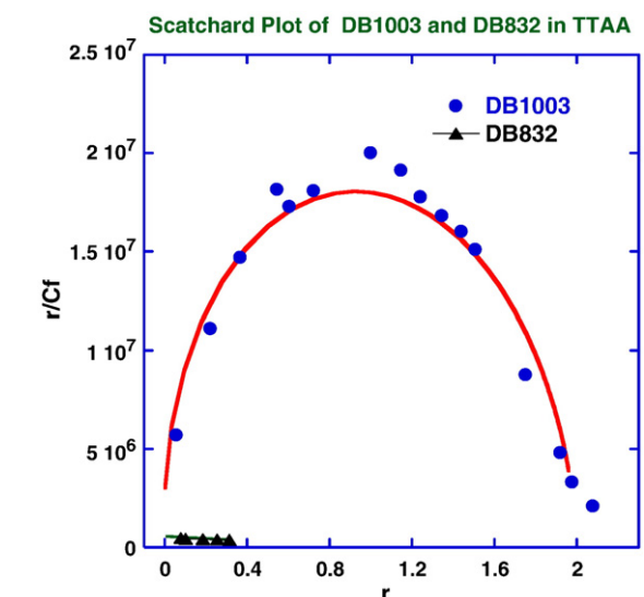
Fig. 6. Scatchard plots of the results for binding of DB1003 and DB832 to TTAA.
