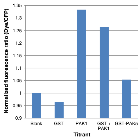
Fig. 5. CFP-PAcKer-derived biosensor has a lower response with the PAK5 kinase domain. PAK1 kinase domain and GST-PAK5 kinase domain at 1 μM was titrated into biosensor. For a good comparison, GST alone at 1 μM or equimolar PAK1 kinase domain and GST (1 μM each) were also titrated into assay mixture containing the biosensor. “Blank” refers to 200 nM of the biosensor alone in assay buffer.
