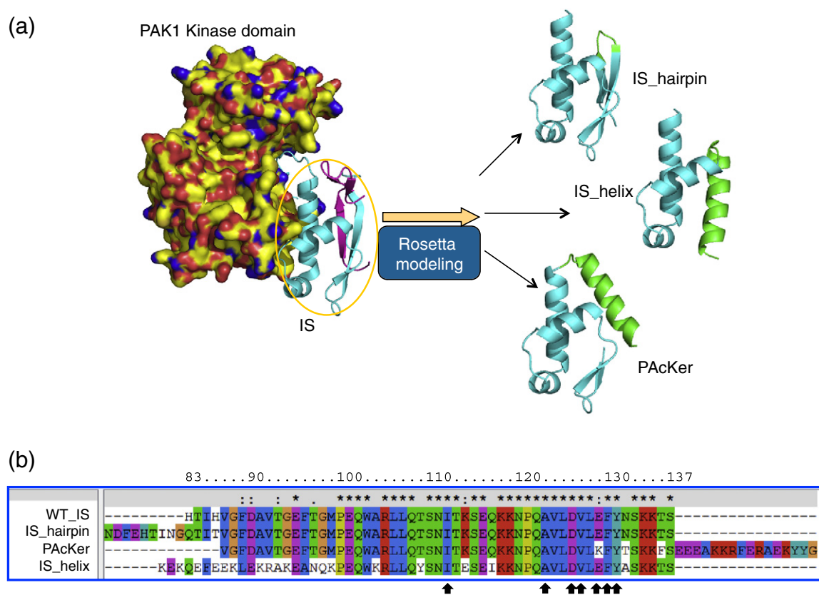
Fig. 1. Structural and sequence comparison of the designs. All the designs were based on the IS domain (IS, cyan), which interacts with the C lobe of the PAK1 kinase domain (yellow). In the crystal structure, PAK1 forms a homodimer in an autoinhibited conformation with a \beta -strand from one IS domain interacting with the partner IS domain (magenta). The rest of the partner is not displayed for clarity. (a) Three alternative designs were tested, “IS_hairpin,” “IS_helix,” and “PAcKer.” The new structural elements added to each variant are shown in green. The cyan regions were left largely intact except for some point mutations that allowed better packing with the new structural elements. (b) Multiple sequence alignment of the variants shows that the new structural elements were at the N-terminus or C-terminus, while the residues involved in binding to the kinase domain were left unmutated (black arrows). The residue numbering is based on the primary sequence of full-length PAK1.
