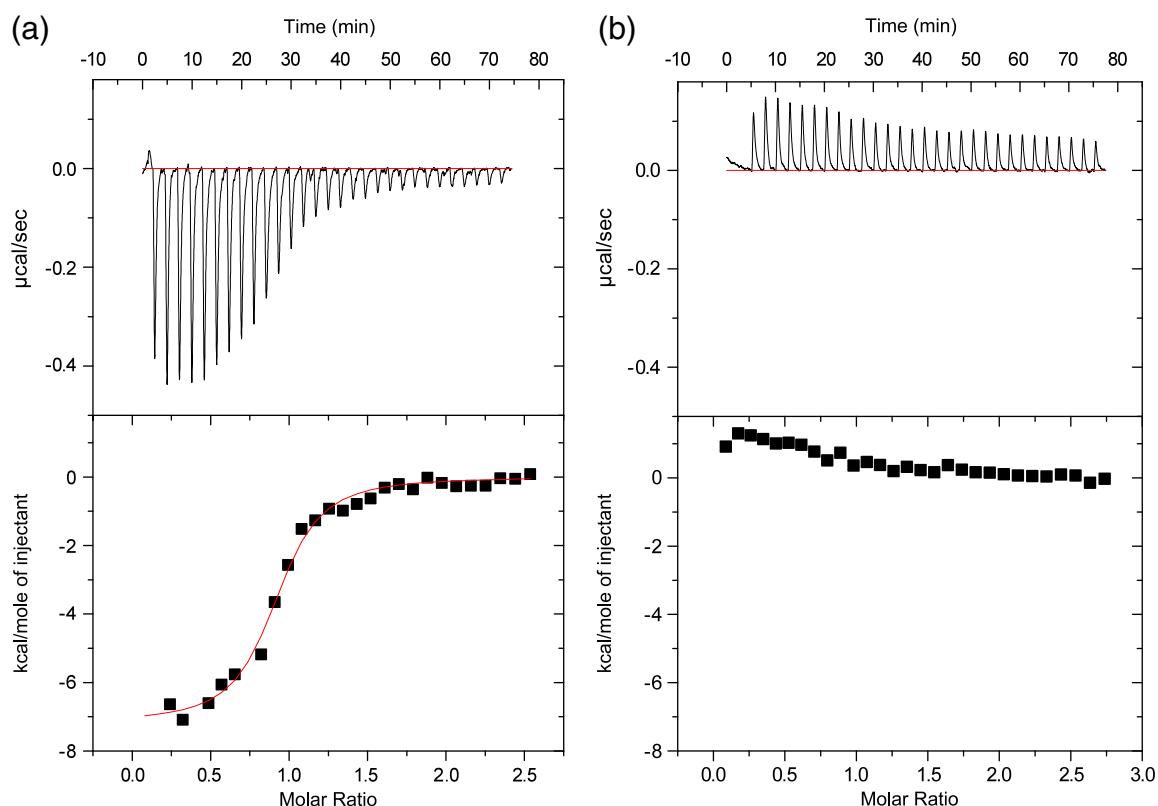
Fig. 3. ITC assays to determine the binding affinities of CFP-PacKer against active and autoinhibited conformations of PAK1. (a) PAK1 kinase domain (208 μM; model for active conformation) was titrated against 18 μM CFP-PacKer. An equilibrium dissociation constant of 400 nM was observed with a molar ratio of ~1. (b) PAK1 full length (262 μM; model for “closed” autoinhibited form) was titrated against 21 μM CFP-PacKer. The titration failed to show any appreciable heat released or absorbed. The data sets were drawn on similar scale for comparison.
