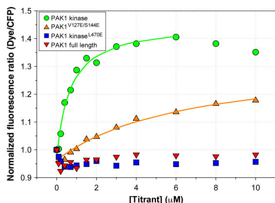
Fig. 4. Biosensor derived from CFP-PAcKer by conjugation with a solvent-sensitive merocyanine dye undergoes fluorescence increase in the presence of PAK1 kinase domain. A net gain of ~40% in the normalized fluorescence ratio was observed in the case of PAK1 kinase domain when it was titrated in 200 nM of biosensor. PAK1 kinase L470E and PAK1 full length failed to show any appreciable change in fluorescence ratio. PAK1 V127E/S144E (full-length “open” PAK1) showed an intermediate level of change in fluorescence ratio.
