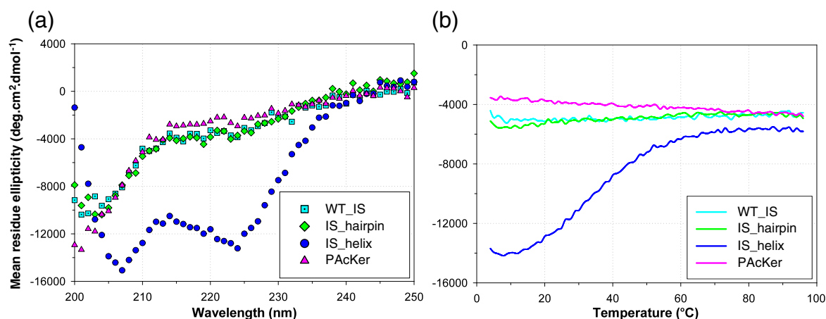
Fig. 2. Structural characterization of computational models and IS domain using CD. (a) IS_helix shows strong helical content. Wild-type IS domain (WT_IS), IS_hairpin and PAcKer are all unfolded. (b) IS_helix shows a modest cooperative thermal denaturation at 222 nm.
