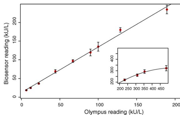
Figure 3 Calibration curve of sAA biosensor. The standard curve is in triplicate and derived from results for sAA serially diluted with stripped saliva and 1% BSA (inset graph). The error bars indicate the standard deviations.
