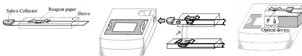
Figure 2 The saliva collector (a) is placed under the tongue, allowed to saturate with saliva ( \approx 10 s) and inserted into the reader (b). Raising the lever transfers the saliva sample onto the reagent paper containing the chromogenic substrate (b). After 10 s, reflectance of the product is measured photometrically at 430 nm (c) and provided as an optical readout.
