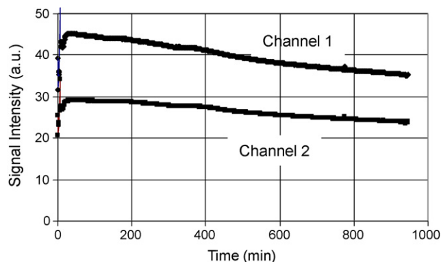
Fig. 5. Bleaching: stability of the fluorophore on the sensor surface over time with repeated laser pulses every 1 min.
