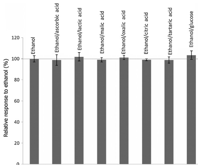
Fig. 6. Comparison of the ethanol biosensor response ( n=3 ) in the absence and in the presence of possible interferents (1:1 ethanol:interferent molar ratio). Measurements were performed at 23 ± 2 °C in 5 mM phosphate buffer pH 7.2 for 50 \mu M ethanol.
