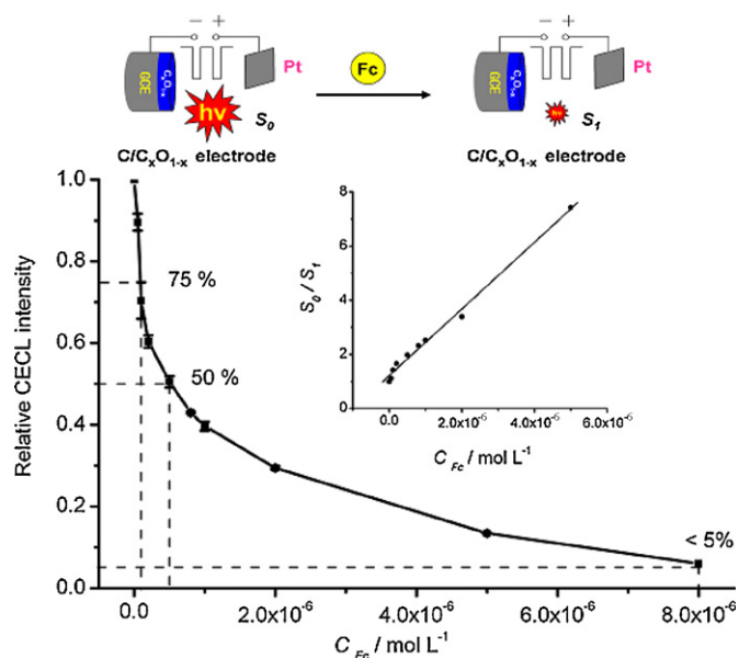
Fig. 1. Quenching effect of Fc on cathodic ECL intensity at C/C_xO_{1-x} electrode. Pulse amplitude: -16\text{ V} (vs. \text{Ag}/\text{AgCl} ), pulse width: 0.4\text{ ms} , duration time: 9.6\text{ ms} and total time: 20\text{ s} . Insert: intensity Stern–Volmer quenching plot for cathodic ECL at C/C_xO_{1-x} electrode by Fc. Solution: 0.2\text{ M} BBS ( \text{pH } 8.0 ) containing 0.1\text{ M} \text{Na}_2\text{SO}_4 and 1\text{ mM} \text{K}_2\text{S}_2\text{O}_8 .
