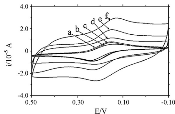
Fig. 2. Cyclic voltammograms of 1.0 mmol/L [\text{Fe}(\text{CN})_6]^{3-/4-} in 0.1 mol/L KCl at (a) bare Au, (b) Au/MPA, (c) Au/MPA/CA-GNP, (d) Au/MPA/(CA-GNP/SPAN), (e) Au/MPA/(CA-GNP/SPAN) 2 and (f) Au/MPA/(CA-GNP/SPAN) 3 .
