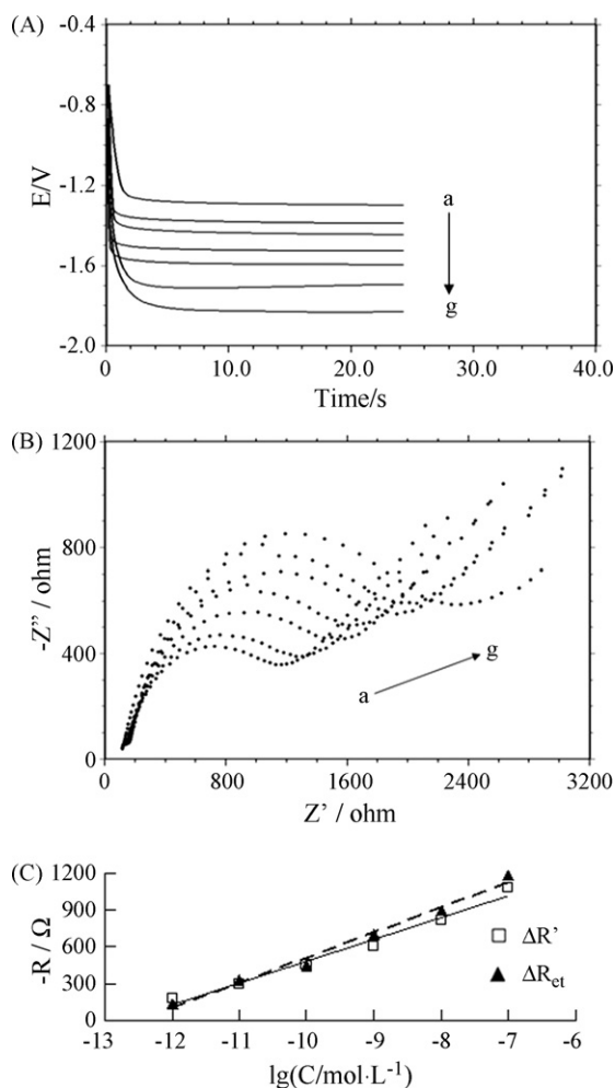
Fig. 6. (A) Chronopotentiometric curves and (B) Nyquist diagrams of 2.0 mmol/L [\text{Fe}(\text{CN})_6]^{3-/4-} recorded at (a) Au/MPA/(CA- \text{G}_{\text{NP}} /SPAN) 3 /CA- \text{G}_{\text{NP}} /ssDNA, and after hybridization with different concentrations of PAT gene sequence (mol/L): (b) 1.0 \times 10^{-12} , (c) 1.0 \times 10^{-11} , (d) 1.0 \times 10^{-10} , (e) 1.0 \times 10^{-9} , (f) 1.0 \times 10^{-8} and (g) 1.0 \times 10^{-7} . (C) The comparison for plots of \Delta R' and \Delta R_{et} versus logarithm of PAT gene fragment concentration.
