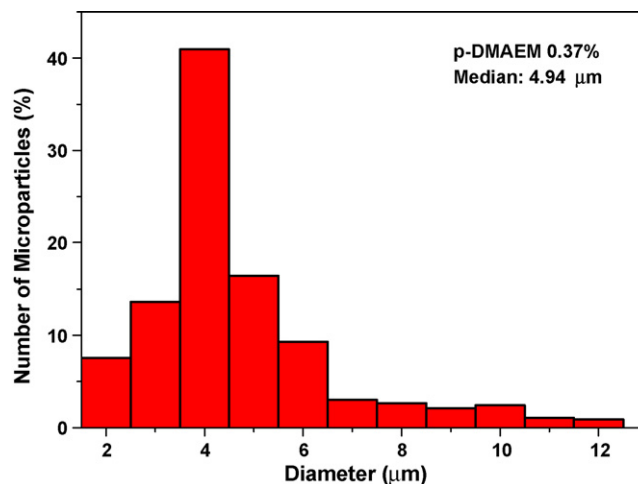
Fig. 2. Size distribution of the p-DMAEM microparticles with entrapped GOx, in phosphate buffer pH 6.0 and 25 ^{\circ}\text{C} .
