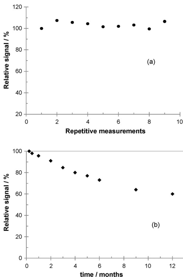
Fig. 9. (a) Amperometric response repeatability of a single LTV-SPE toward catechol quantification, in a aqueous solution containing 50 catechol \mu\text{M} in 0.1 M acetate buffer, pH 4.7 and 30 °C, applying -0.30\text{ V} . RSD=2.73. (b) Stability measured as a plot of the relative signal as a function of elapsed time under dry buffer-less 4 °C storage conditions.
