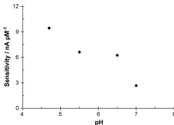
Fig. 6. pH dependence of LTV-SPE response toward hydroquinone at -0.30\ \text{V} and 30^\circ\text{C} .
