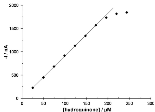
Fig. 5. Calibration plot for the LTV-SPE recorded with hydroquinone in 0.1\ \text{M} acetate buffer at -0.30\ \text{V} , pH 4.7 and 30^\circ\text{C} .
