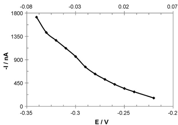
Fig. 4. Effect of applied potential on the LTV-SPE response to hydroquinone 100\ \mu\text{M} in 0.1\ \text{M} acetate buffer at pH 4.7 and 30^\circ\text{C} . In the second X-axis it is reported de potential values vs. a commercial \text{Ag}/\text{AgCl}/\text{Cl}^-_{(\text{aq})}\ 3\ \text{M} electrode.
