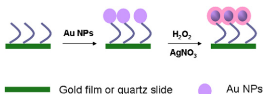
Fig. 1. Schematic illustration for the fabrication process of the AuAg bimetallic nanoparticles film.
