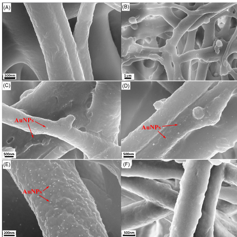
Fig. 2. Scanning electron micrographs of eggshell membranes after they had contacted with 0.76 mM HAuCl 4 solutions for 1.5 h under various pHs: (A) a natural eggshell membrane for comparison, (B) 3.0, (C) 4.0, (D) 5.0, (E) 6.0, and (F) 7.0.
