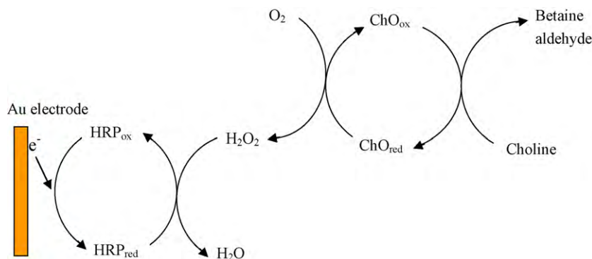
Scheme 2. The reaction illustration of the Au/PtpolyCD/ADA/E electrode for the detection of choline in solution.
