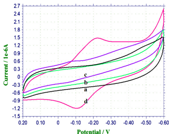
Fig. 2. CVs of bare Au electrode (a), ATP/Au (b), diazo-ATP/Au (c), and Th/diazo-ATP/Au (d) in 0.1 M PBS (pH 6.0) at a scan rate of 50 mV s -1 .
