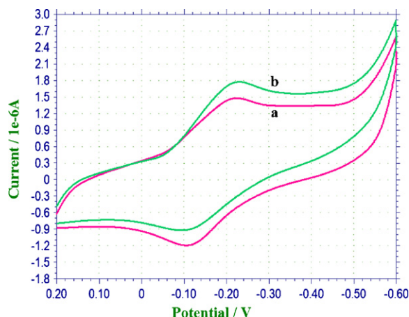
Fig. 4. CVs of Th/diazo-ATP/Au (a) without H 2 O 2 and (b) with 1 mM H 2 O 2 in 0.1 M PBS (pH 6.0) at a scan rate of 50 mV s -1 .
