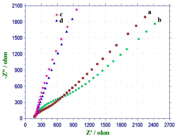
Fig. 3. EIS for bare Au electrode (a), ATP/Au (b), diazo-ATP/Au (c), and Th/diazo-ATP/Au (d) in a solution of 0.1 M KCl containing 1.0 mM Fe(CN) 6 3- and 1.0 mM Fe(CN) 6 4- .
