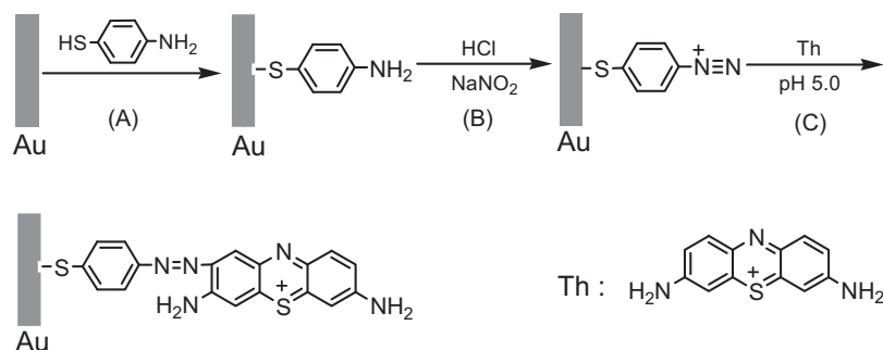
Fig. 1. Schematic representation of the fabrication of \text{H}_2\text{O}_2 sensor based on covalent immobilization of Th on self-assembled diazo-ATP modified Au electrode by diazotization-coupling reaction.
