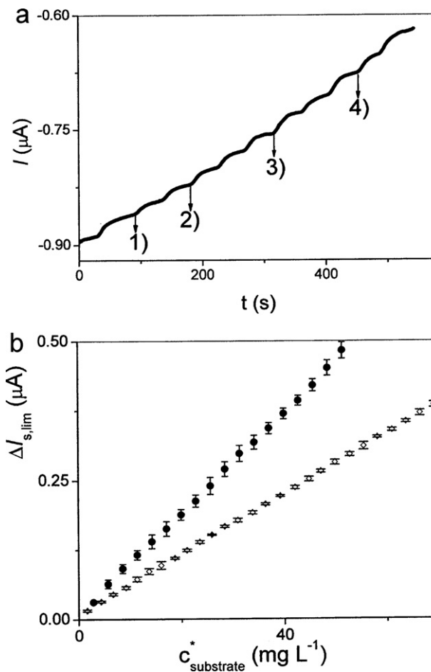
Fig. 4. (a) Steady-state current responses on the addition of different t-Res concentrations in a reaction medium under stirring containing 240 IU \text{mL}^{-1} PBHR + 50 \mu\text{mol L}^{-1} \text{H}_2\text{O}_2 in PBS pH 7.00 measured with a dialysis membrane covered PBHR-Fc-MWCNT+MO (10-3-45) biosensor. c_{\text{t-Res}}^* : (1) 5.7 \mu\text{mol L}^{-1} ; (2) 11.4 \mu\text{mol L}^{-1} ; (3) 20.0 \mu\text{mol L}^{-1} and (4) 28.5 \mu\text{mol L}^{-1} . (b) Calibration curves defined as the differences between the base and the steady-state currents, \Delta I_{s,\text{lim}} , with corresponding error bars, as a function of c_{\text{t-Res}}^* ( \bullet ) and c_{\text{CA}}^* ( \diamond ), respectively, under the same experimental conditions as in (a).
