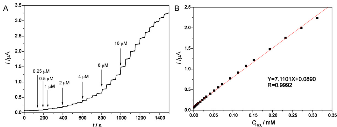
Fig. 4. (A) Chronoamperometric response of the biosensor to successive additions of H 2 O 2 in 0.1 mol L -1 PBS (pH = 7.0) containing 0.4 mmol L -1 HQ. (B) The calibration curve of the currents on the concentration of H 2 O 2 .
