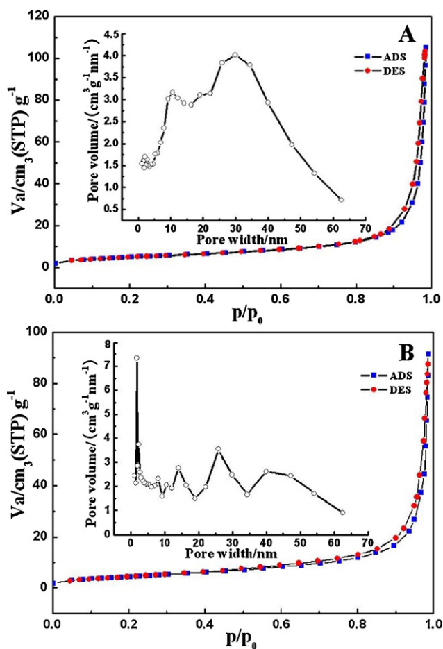
Fig. 2. Nitrogen adsorption (ADS)/desorption (DES) isotherms of \text{Fe}_3\text{O}_4 microsphere (A) and \text{Fe}_3\text{O}_4 -GR mixture (B). Inset is the corresponding pore size distribution.
