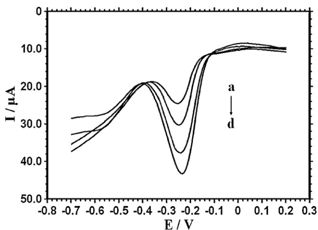
Fig. 4. Differential pulse voltammograms of 4.0 \times 10^{-5} mol/L MB on (a) dsDNA/CTS/CILE, (b) dsDNA/CTS/ Fe_3O_4 /CILE, (c) dsDNA/CTS/GR/CILE and (d) dsDNA/CTS/ Fe_3O_4 -GR/CILE in 50 mmol/L Tris-HCl buffer solution contained 20.0 mmol/L NaCl (pH 7.4).
