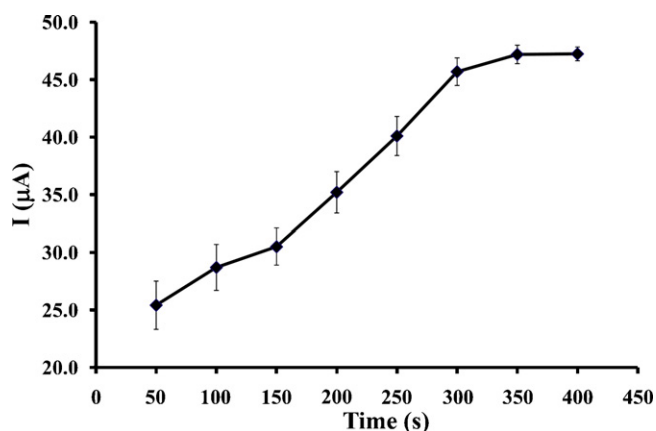
Fig. 6. Effect of accumulation time of Sudan II on the stripping oxidation current in 0.1 \text{ mol L}^{-1} PBS containing 0.1 \mu\text{g mL}^{-1} Sudan II at an open-circuit condition and with stirring. (Error bars show the relative standard deviation, n = 3 .)
