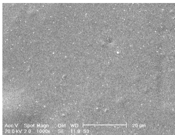
Fig. 7. SEM image of GOD/GNPs/CNTs/nafton film on graphite support.
