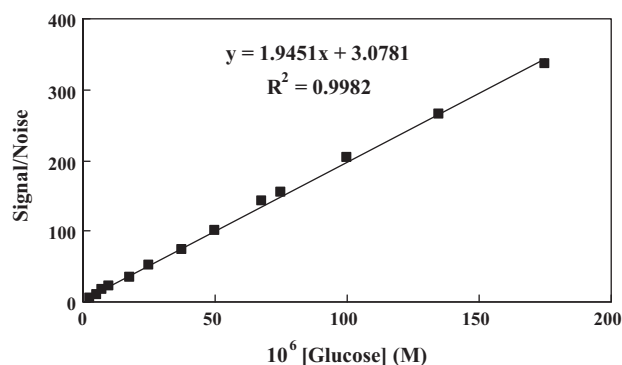
Fig. 10. Calibration curve for glucose determination with nafion/GOD/GNPs/CNTs graphite biosensor. Conditions: [\text{Flu}] = 1.90 \times 10^{-4} \text{ mol L}^{-1} , [\text{sodium salicylate}] = 1.0 \times 10^{-6} \text{ mol L}^{-1} , [\text{TCPO}] = 7.00 \times 10^{-4} \text{ mol L}^{-1} .
