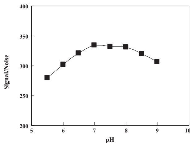
Fig. 8. Effect of pH on signal/noise ratio, conditions: [\text{Flu}] = 1.90 \times 10^{-4} \text{ mol L}^{-1} , [\text{sodium salicylate}] = 1.0 \times 10^{-6} \text{ mol L}^{-1} , [\text{TCPO}] = 7.00 \times 10^{-4} \text{ mol L}^{-1} , [\text{glucose}] = 1.20 \times 10^{-4} \text{ mol L}^{-1} .
