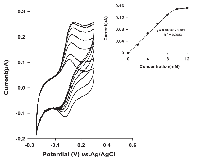
Fig. 6. Cyclic voltammograms of MWCNTs/IL/Ox-P(NAD + ) modified GC electrode in PBS (pH 8.8) containing 1 × 10 -3 mol L -1 of each NAD + and ADH compounds at different concentrations of ethanol and scan rate of 10 mV s -1 (from inner to outer) 0, 2, 4, 6, 8, 10 and 12 (× 10 -3 mol L -1 ). Inset is the plot of catalytic current vs. ethanol concentrations.
