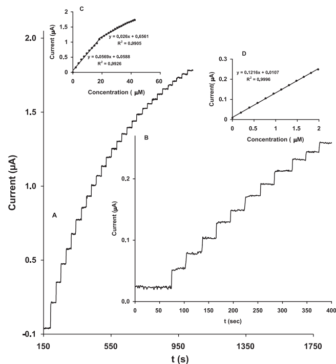
Fig. 5. (A) Amperometric response of rotating MWCNTs/IL/Ox-P(NAD + ) modified GC electrode to successive additions of 2 \times 10^{-6} \text{ mol L}^{-1} NADH, at applied potential of 0.1 \text{ V} , PBS (pH 8.8) and rotation speed is 400 \text{ rpm} . (B) Successive additions of 2 \times 10^{-7} \text{ mol L}^{-1} NADH. (C and D) plots of chronoamperometric current vs. NADH concentration.
