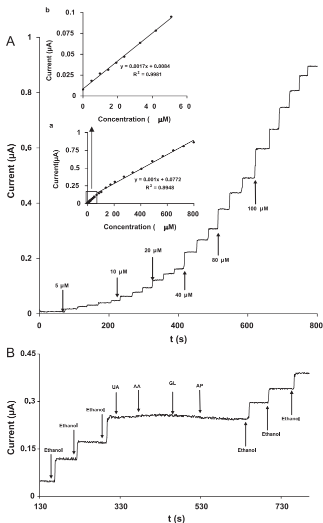
Fig. 7. (A) Chronoamperometric response of MWCNTs/IL/Ox-P(NAD + ) modified GC electrode in 1 × 10 -3 mol L -1 NAD + and 1 × 10 -3 mol L -1 ADH, 0.1 mol L -1 PBS (pH 8.8) on injecting different concentrations of ethanol at working potential of 0.1 V vs. Ag/AgCl. Inset (a): plot of amperometric response vs. ethanol concentrations and inset (b) is the enlarged view of the defined segment in inset a. (B) Amperometric response of the MWCNTs/IL/Ox-P(NAD + ) modified GC electrode in 0.1 mol L -1 PBS (pH 8.8) containing 5 × 10 -5 mol L -1 ethanol, 1 × 10 -3 mol L -1 NAD + and 1 × 10 -3 mol L -1 ADH spiked with UA (0.1 mM), AA (0.1 mM), AP (0.1 mM), and GL (0.1 mM).
