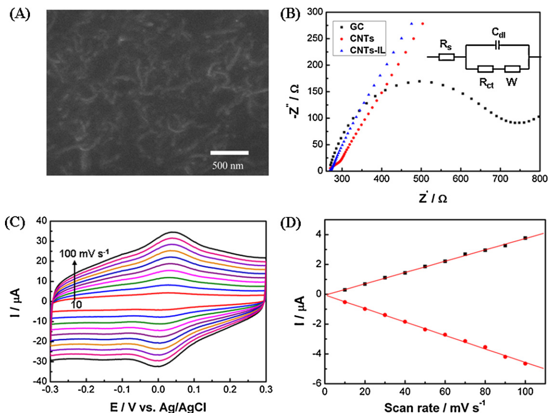
Fig. 1. (A) SEM image of CNTs-IL nanocomposites. (B) EIS of GCE (black), CNTs (red) and CNTs-IL nanocomposites (blue) modified GCEs in 0.02 M KCl solution containing 2.5 mM \text{K}_3[\text{Fe}(\text{CN})_6] and 2.5 mM \text{K}_4[\text{Fe}(\text{CN})_6] . Frequency range: 10^5 –1 Hz. (C) CVs of CNTs-IL/GCE in PBS (pH 7.4) with different scan rates. From inner to outer: 10, 20, 30, 40, 50, 60, 70, 80, 90 and 100 \text{mV s}^{-1} . (D) Anodic (black) and cathodic (red) peak current vs. scan rate. (For interpretation of the references to color in this figure legend, the reader is referred to the web version of the article.)
